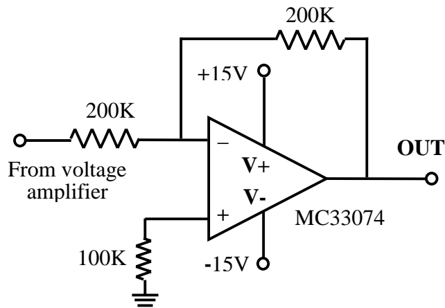
Fig.A-18 Inverting amplifier for load current sensing
