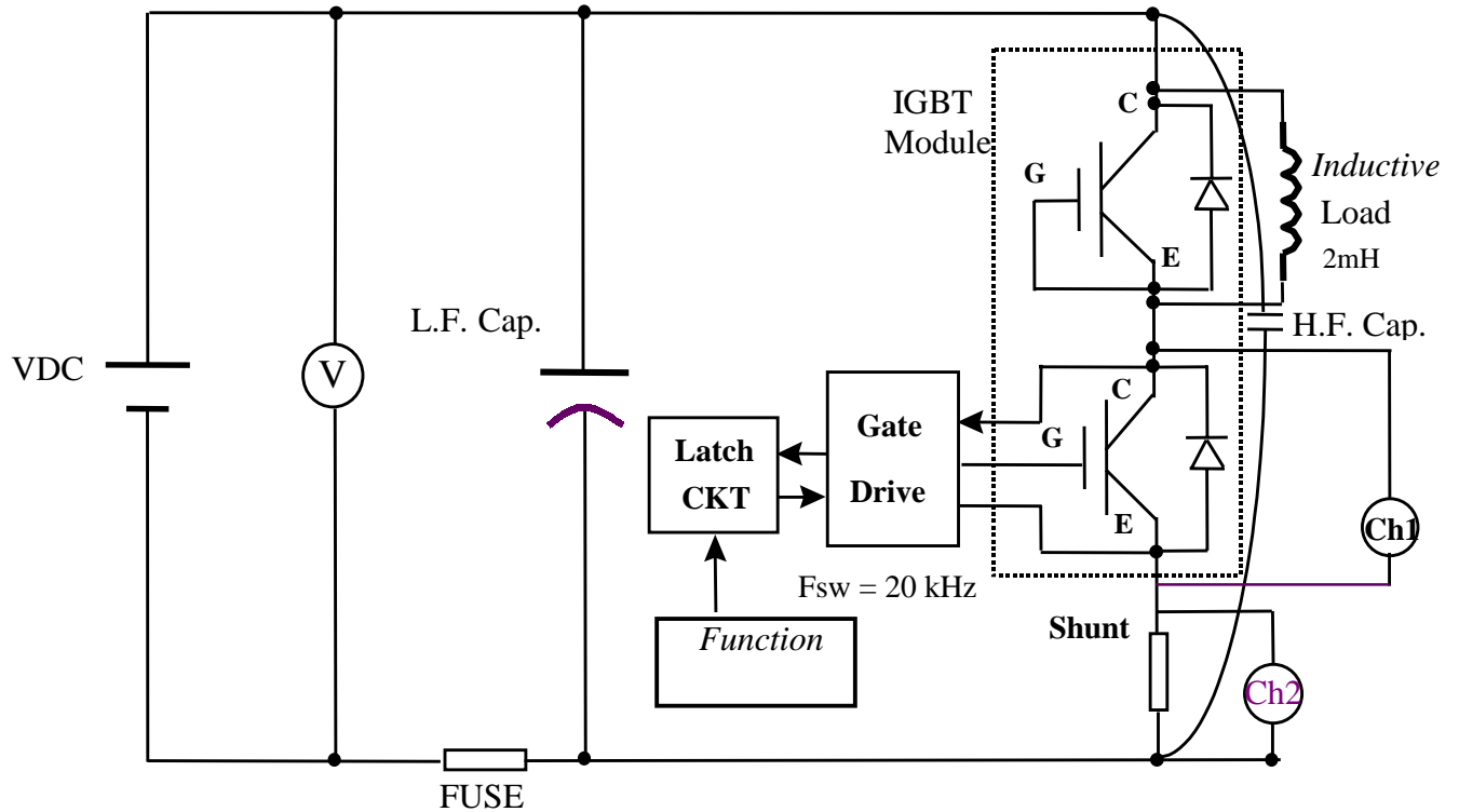
Fig. 3.1 IGBT turn on / turn off testing circuit
