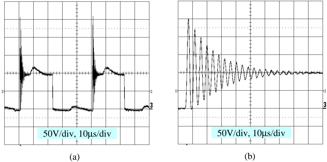
Fig.3.25 Voltage ringing across auxiliary switch
