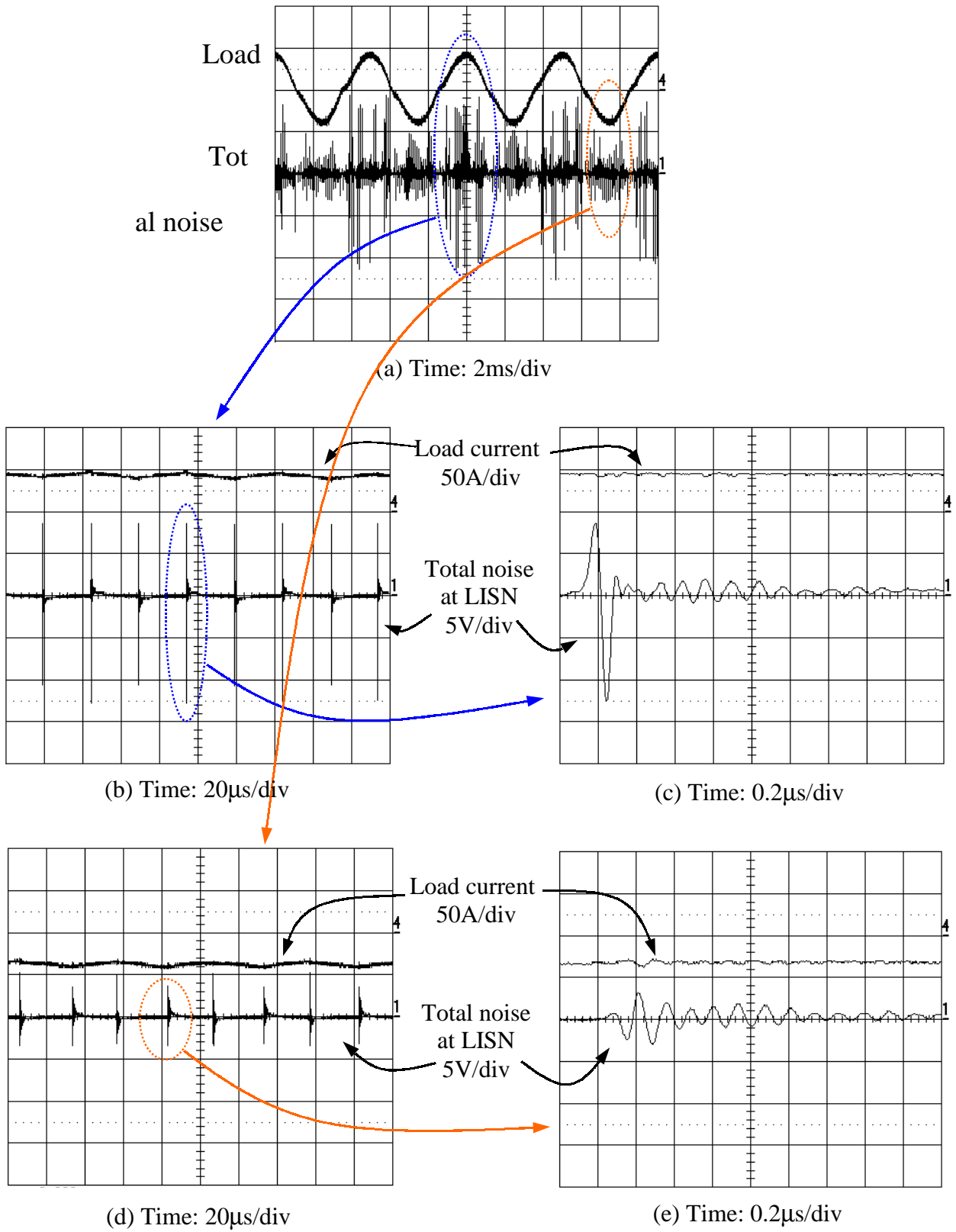
Fig. 3.16 Hard-switching inverter total noise at LISN
