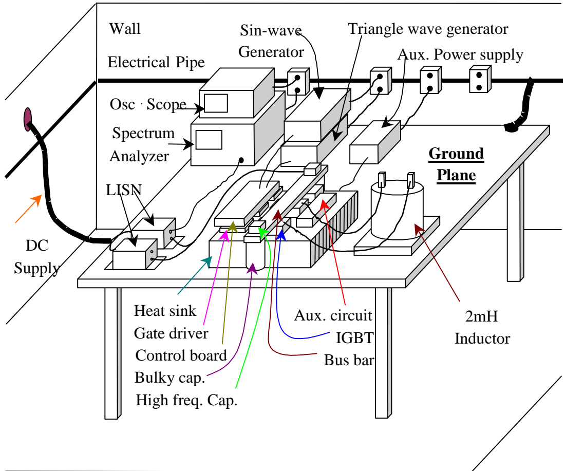
Fig. 2.2 Test setup in EMI room
