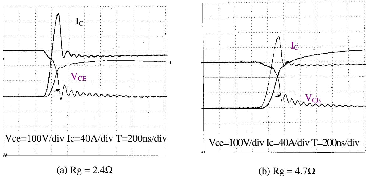
Fig. 3.3 IGBT turn on with different gate resistor
