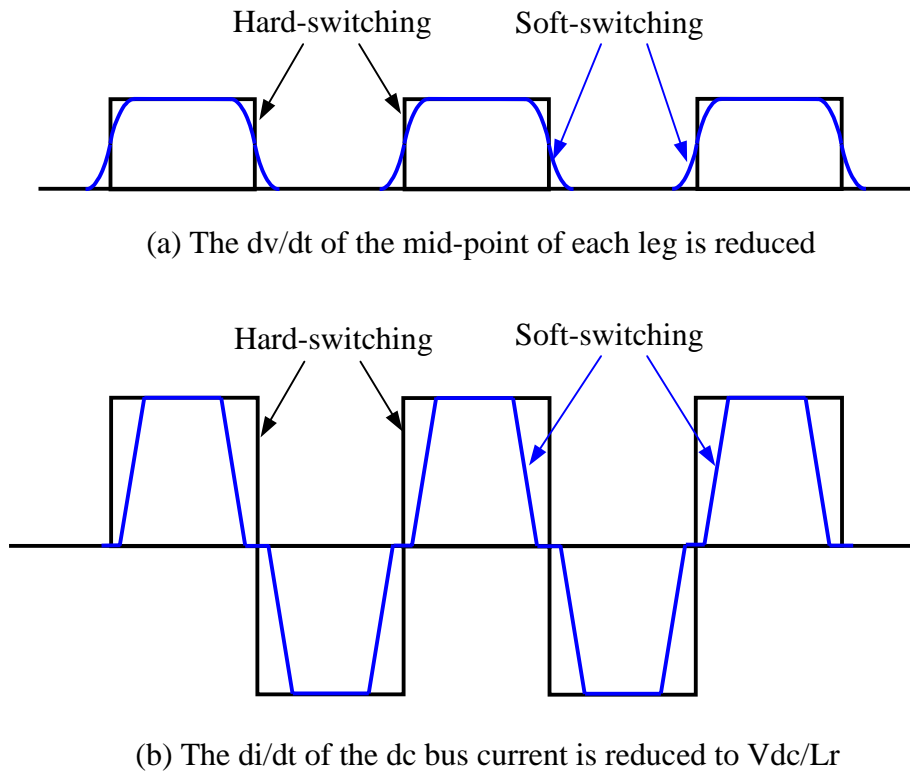
Fig. 3.23 dv/dt and di/dt of the inverter is reduced by soft-switching
