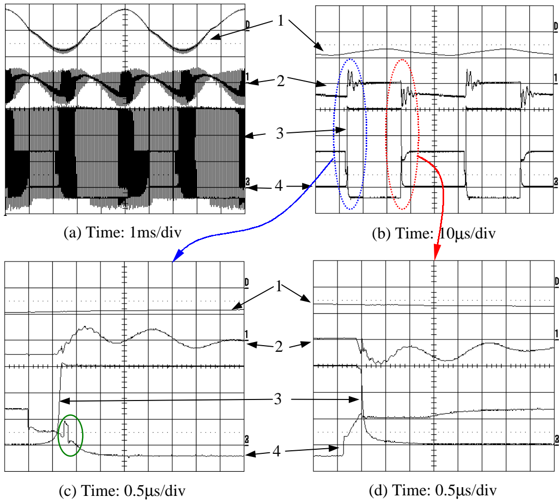
1) Load current 50A/div; 2) dc bus voltage ripple 2V/div; 3) Vce of T3 100V/div; 4) Vge of T3 10V/div
