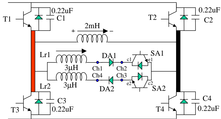
Fig.3.31 Split resonant inductor in the soft-switching inverter
