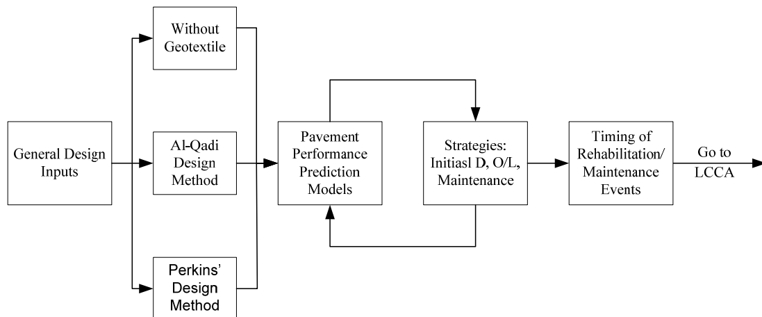
Figure 4-1 Life Cycle Cost Framework- Pavement Performance
