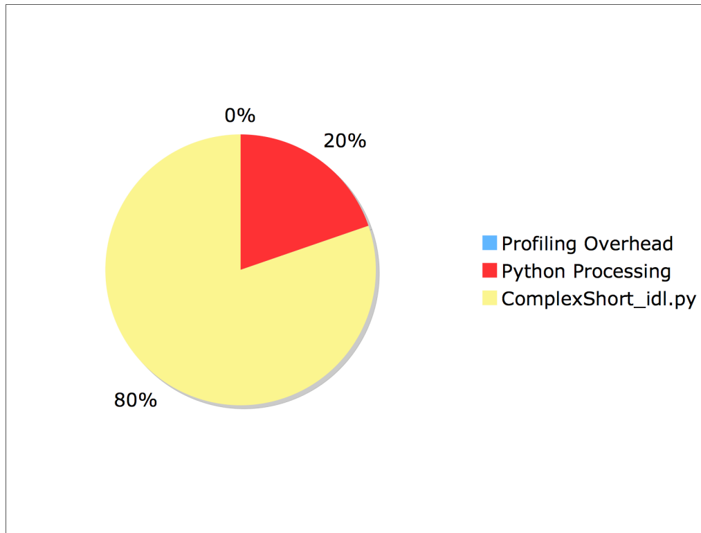
Figure 5.3: Breakdown of Execution Time for Simulation 1. Categorized as Python processing, profiling overhead, and ComplexShort_idl.py
