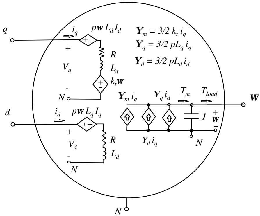
a) Electrical signal model
