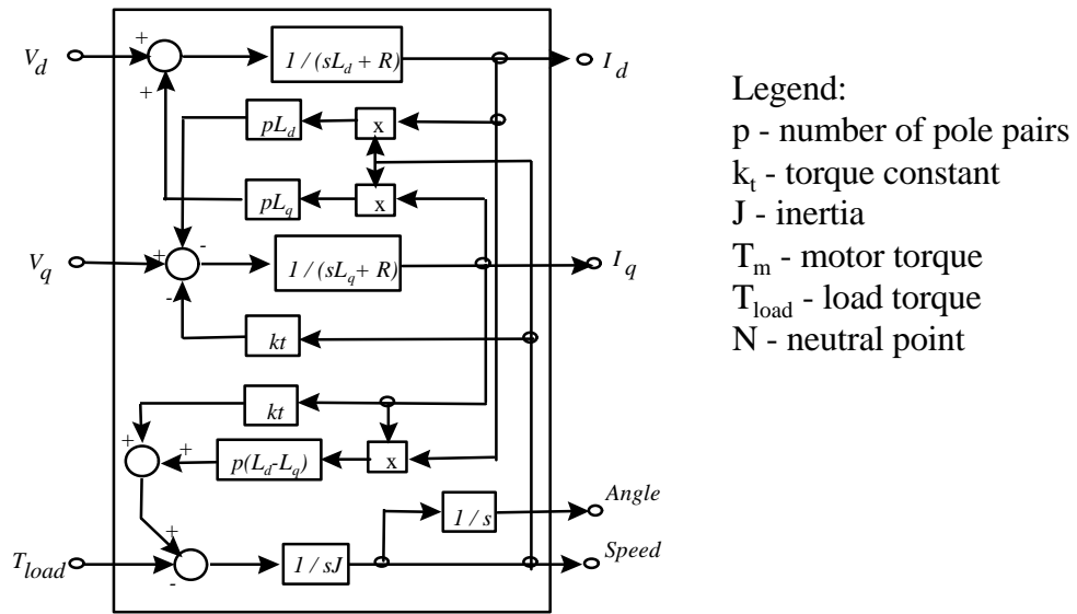
b) Control signal model
