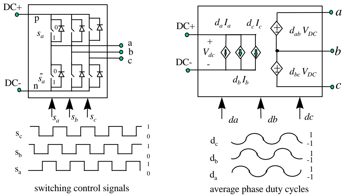
a) Switching model
