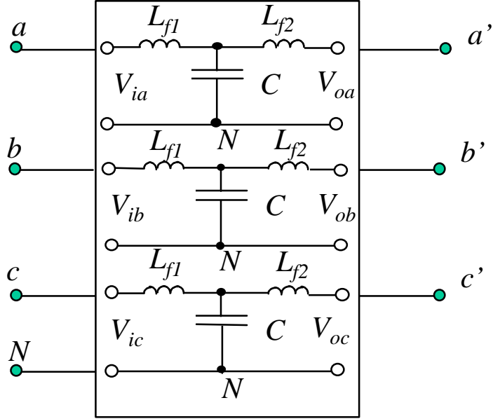
a) Three-phase model
