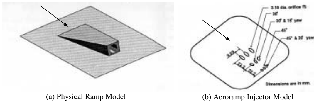
Figure 1.8: Comparison of a Physical Ramp and Aeroramp Injector (Fuller et al., 1996)
