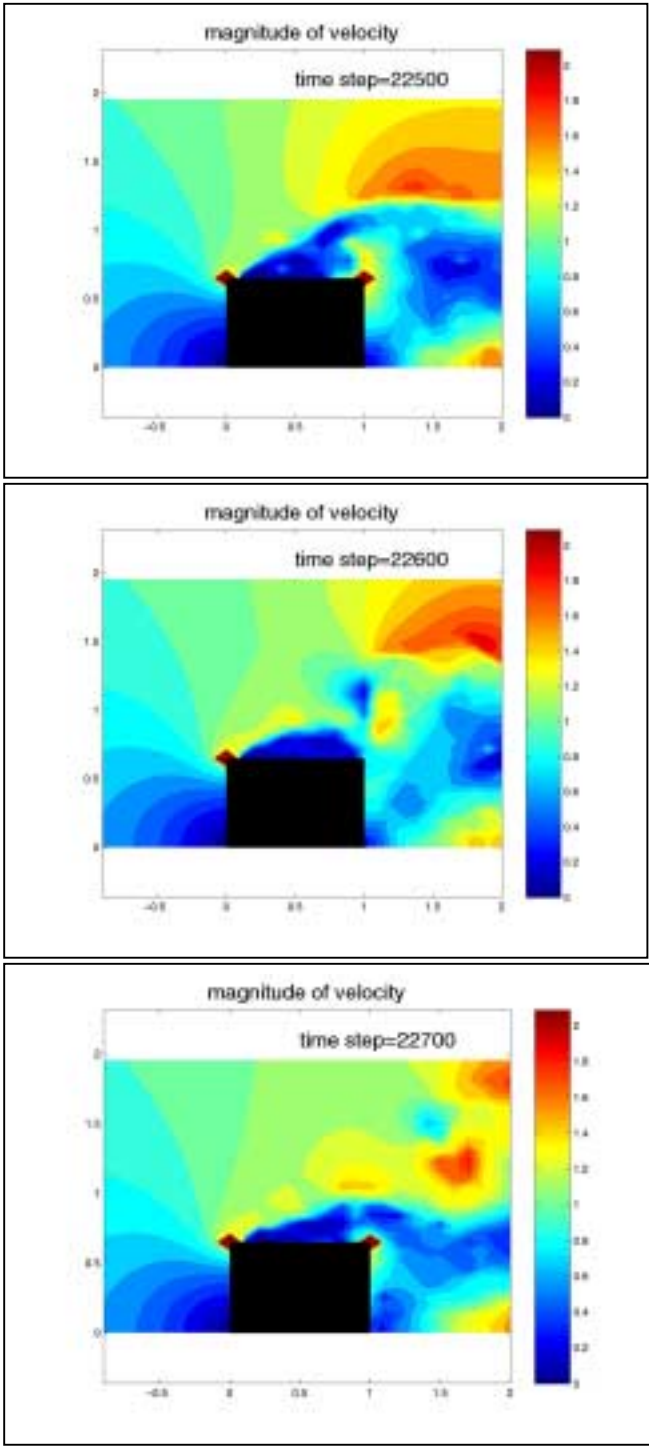
Fig. 4.10 Velocity magnitude
