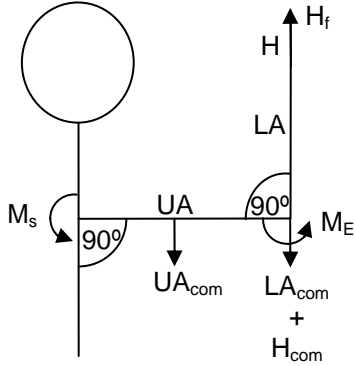
Figure III.2. Shoulder angle free body diagrams
