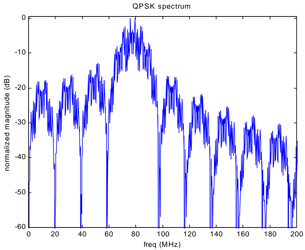
Figure 4.16: QPSK spectrum
