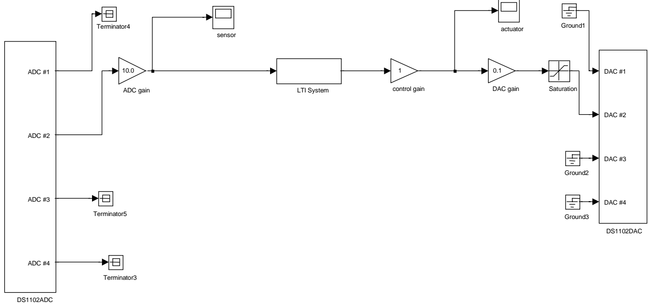
Figure 5.10. SIMULINK block diagram used to implement the PPF controller.
