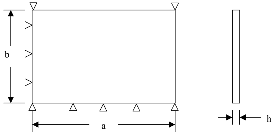
Figure 5.2. Orthographic views of the simply supported steel plate.
