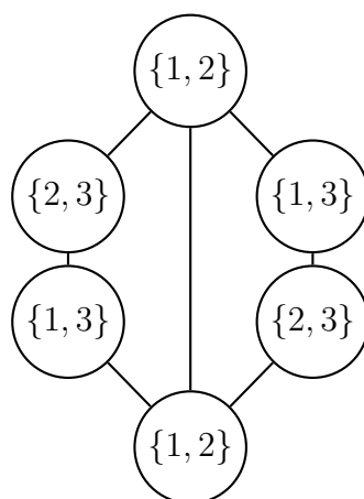
Figure 2.5: A \theta_{a,b,c} graph with a, b \neq 2
