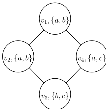
(b) C_4 Case 2
