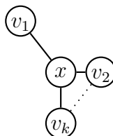
Figure 2.9: Subgraph induced by edges incident with x
