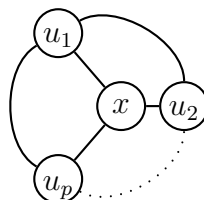
Figure 2.10: Wheel and spokes
