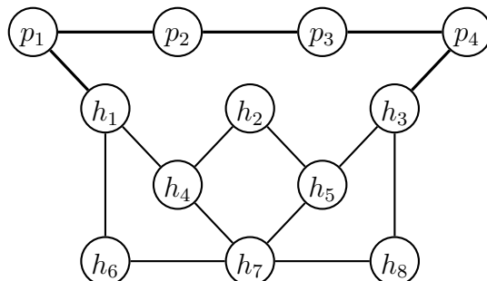
Figure 4.1: P is an ear of H
