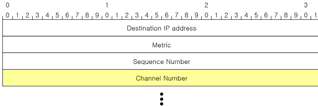
Figure 4.3: DSDV-MC HELLO message.
