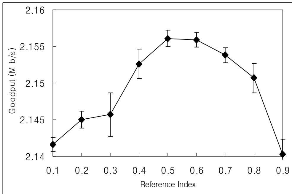
Figure 6.18: Goodput for multiple-hop network for varying reference index.
