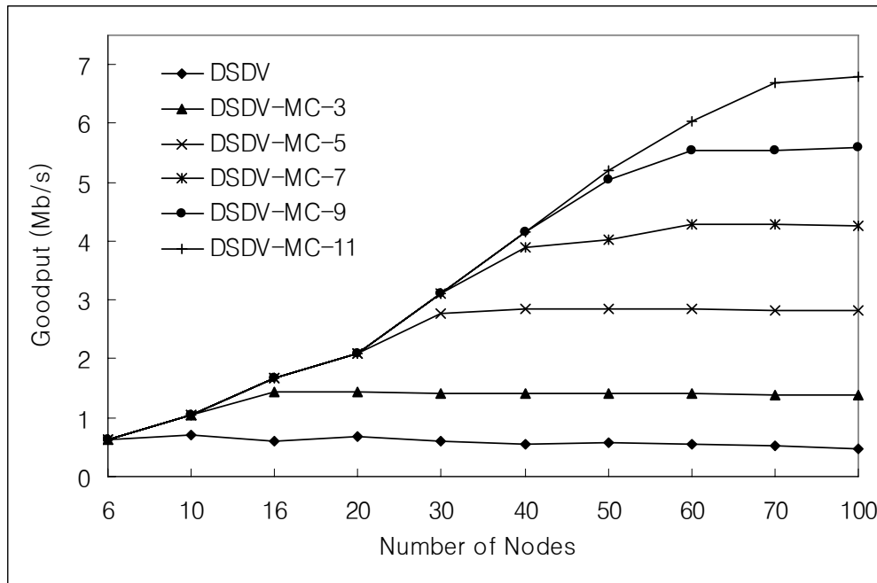
Figure 6.3: Goodput for single-hop network with varying numbers of nodes.
