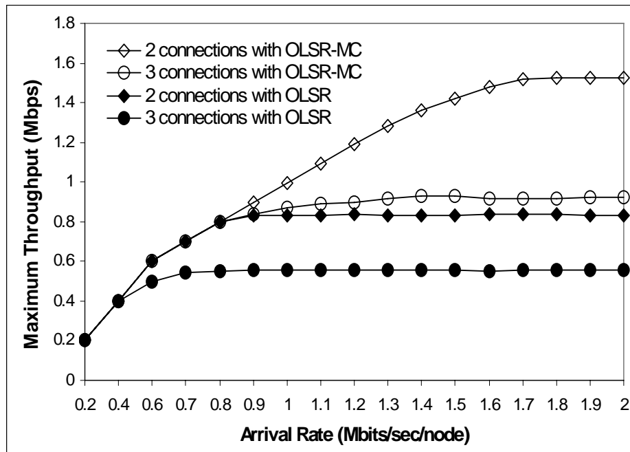
Figure 7.6: Maximum throughput for varying arrival rate.
