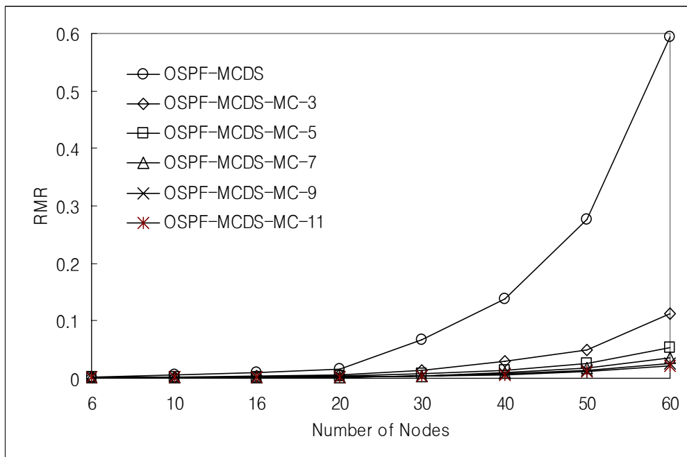
Figure 6.23: RMR for single-hop network for different numbers of channels and different numbers of nodes.
