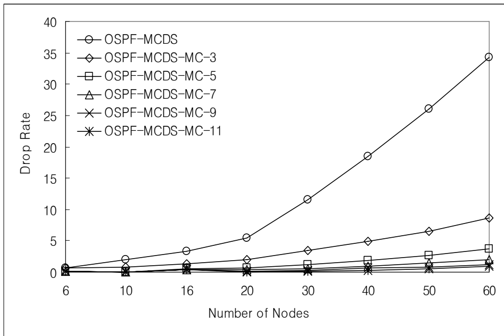
Figure 6.21: Packet drop rate for single-hop network for varying numbers of nodes.
