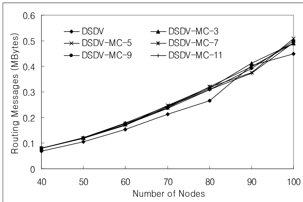
Figure 6.10: Number of routing messages for varying numbers of nodes
