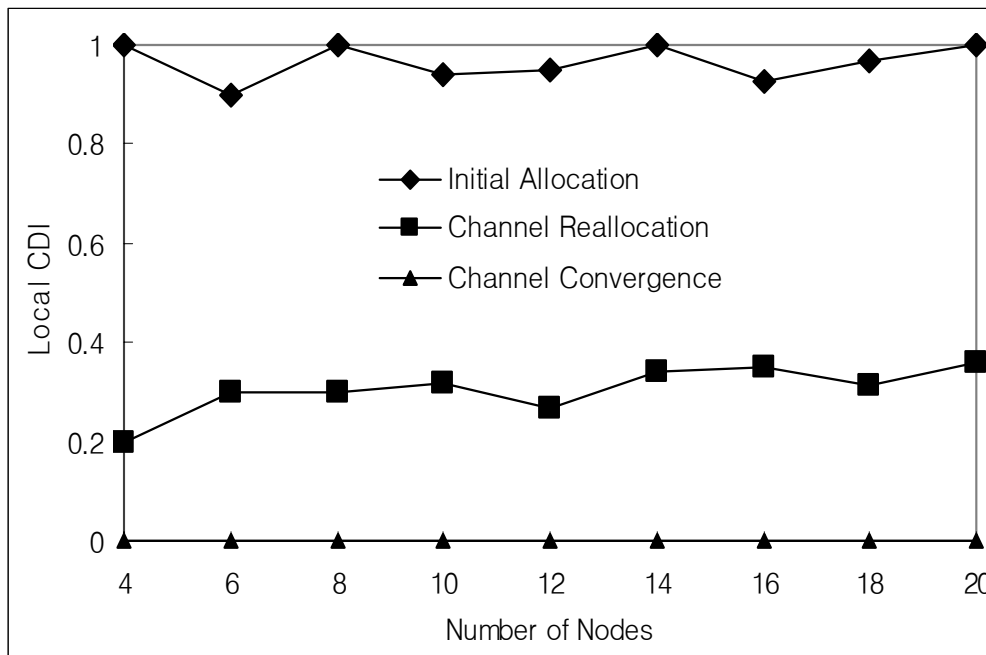
Figure 6.12: CDI for linear network for varying numbers of nodes.
