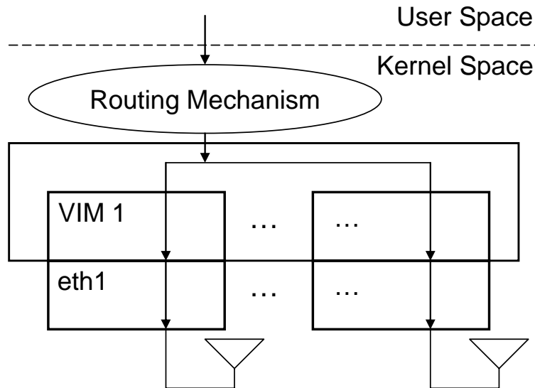
Figure 7.4: Multiple virtual interface scheme.
