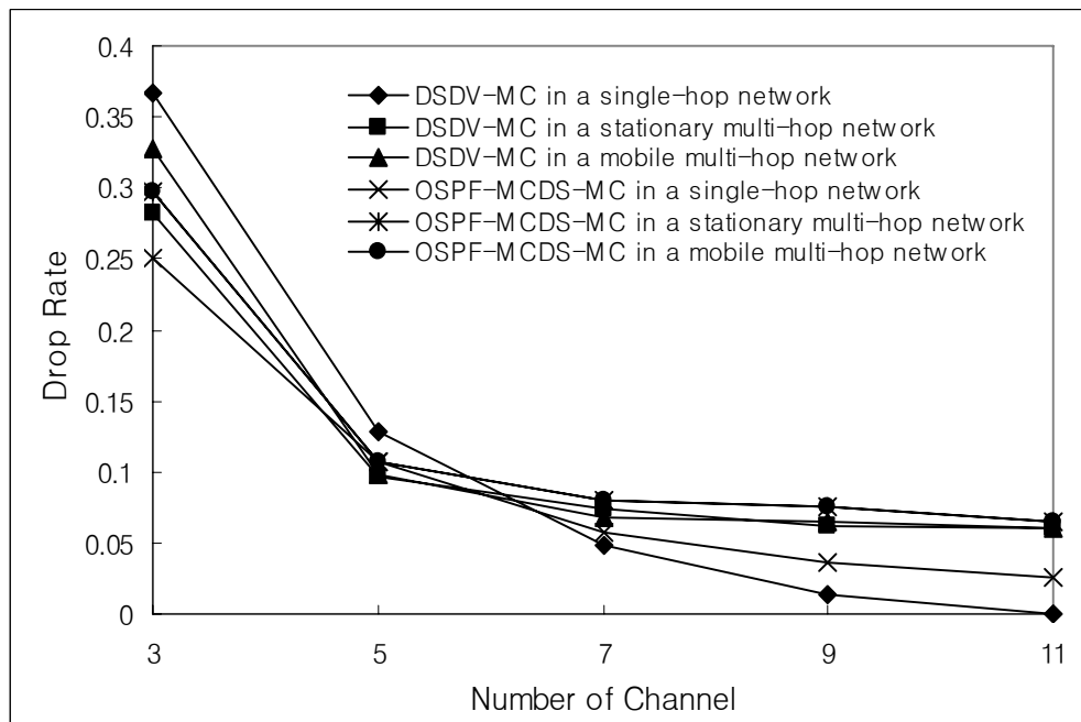
Figure 6.34: Drop rate for varying numbers of channels.
