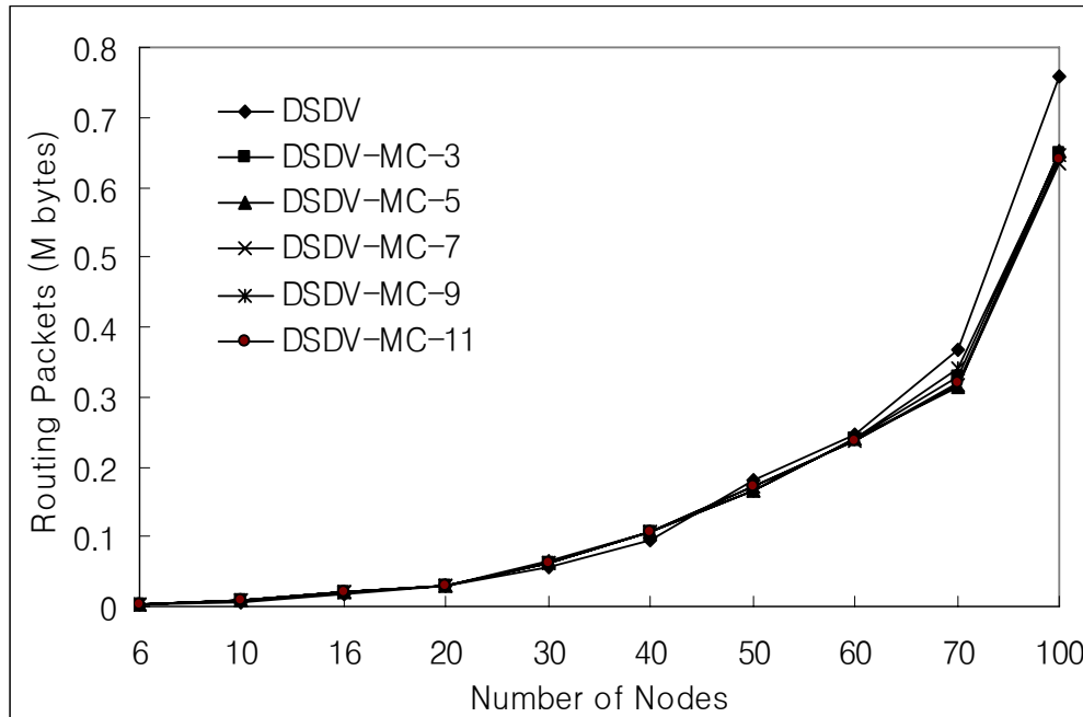
Figure 6.5: Routing packets for single-hop network with varying numbers of nodes.
