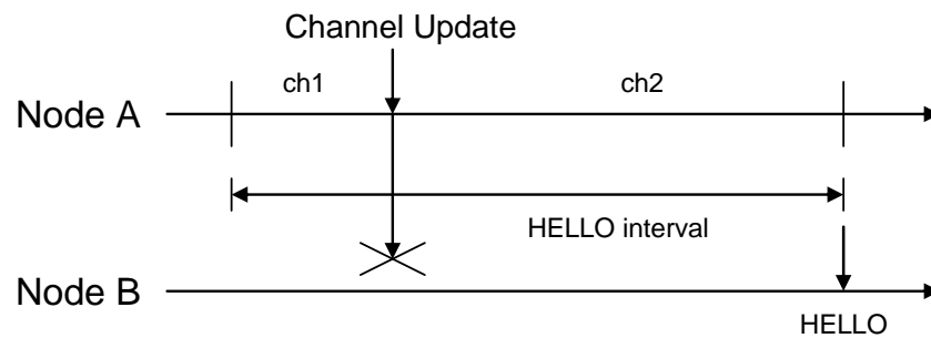
Figure 4.11: Illustration of CU message loss.
