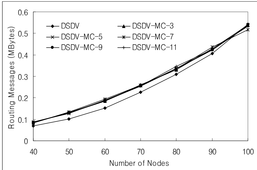
Figure 6.11: Number of routing messages for varying numbers of nodes in a mobile multiple-hop network.
