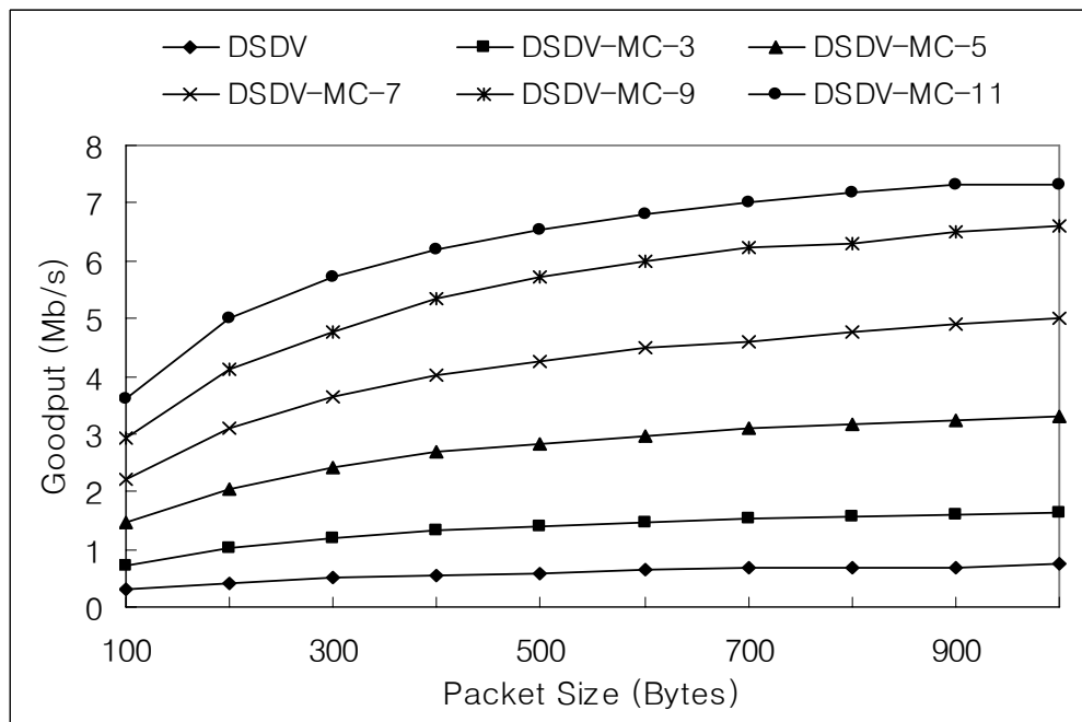
Figure 6.6: Goodput for single-hop network with varying packet size.
