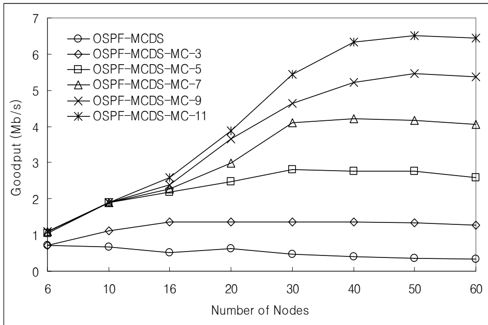
Figure 6.20: Goodput for single-hop network for varying numbers of nodes.
