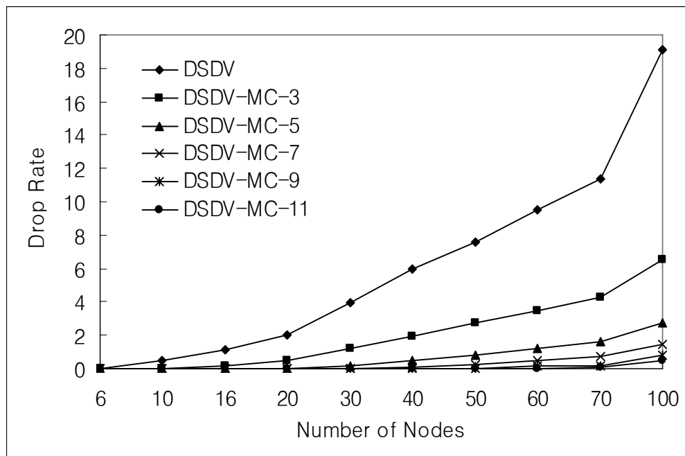
Figure 6.4: Packet drop rate for single-hop network with varying numbers of nodes.
