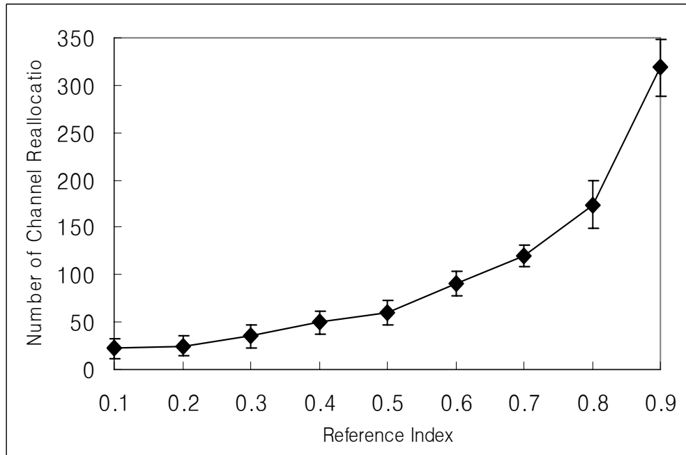
Figure 6.19: Frequency of channel reallocation in a multiple-hop network for varying reference index.
