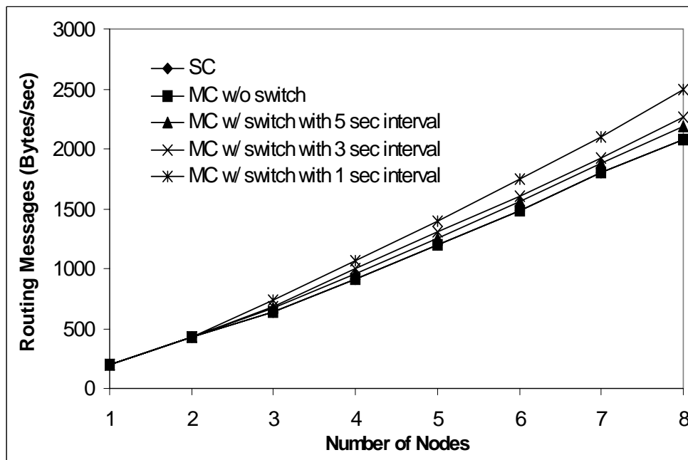
Figure 7.8: Data rate for routing messages for different numbers of nodes.
