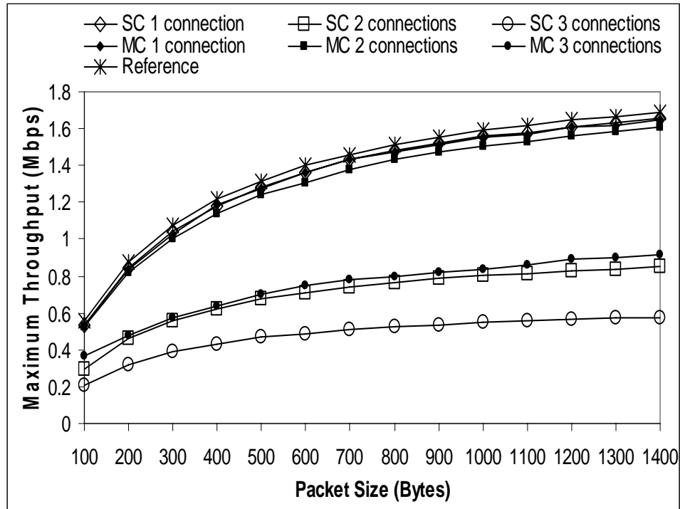
Figure 7.7: Throughput with varying packet size.
