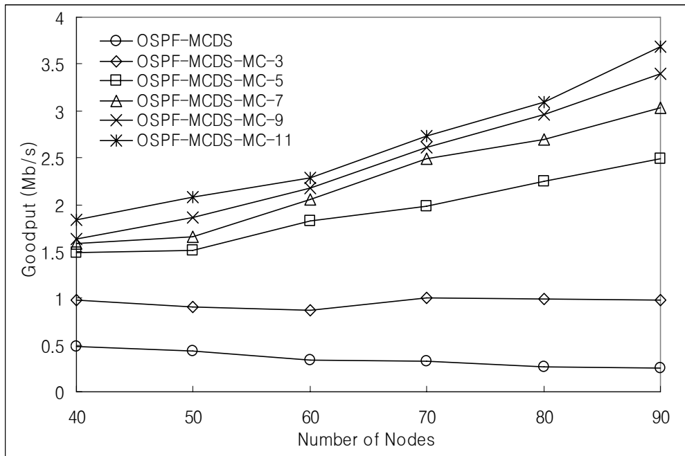
Figure 6.30: Goodput for stationary multiple-hop network for varying numbers of nodes.
