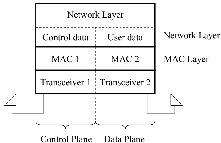
Figure 4.1: Control and data planes at a node with two transceivers.
