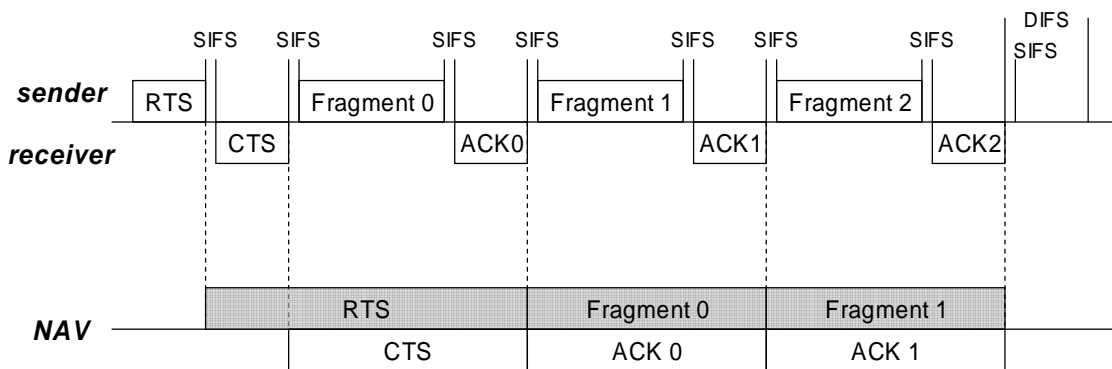
Figure 3.3: NAV setting for a burst of fragments.
