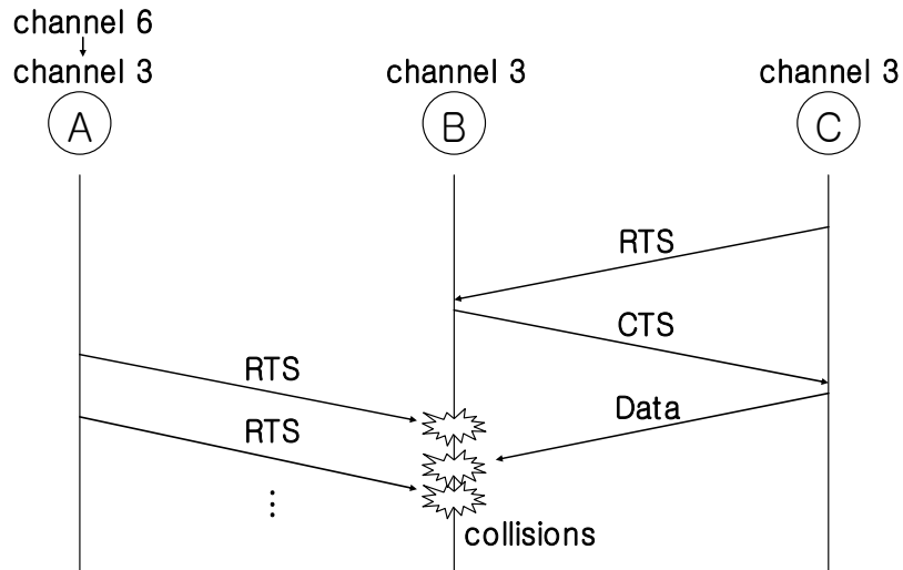
Figure 3.2: Hidden terminal problem under multi-channel networks.
