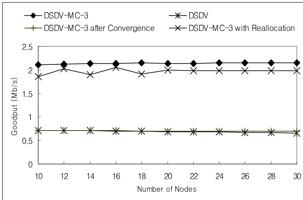
Figure 6.15: Goodput for the single-hop network for varying numbers of nodes.
