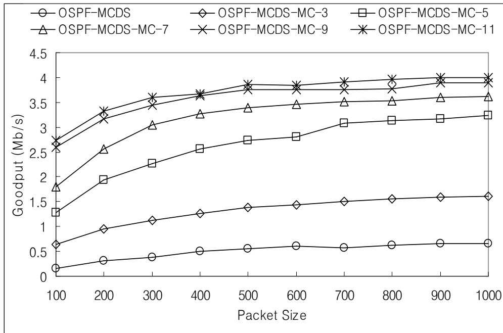
Figure 6.24: Goodput for single-hop network for varying packet size.
