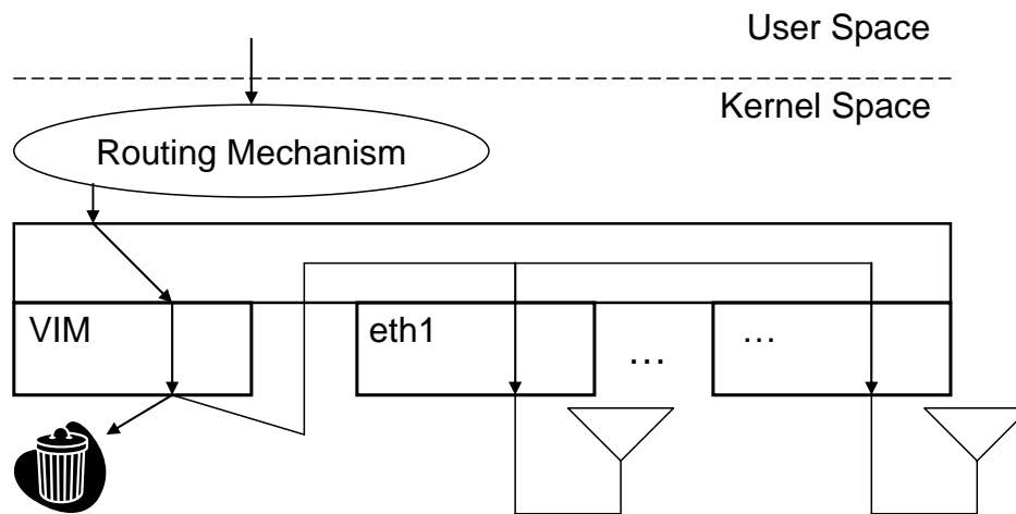
Figure 7.2: Data flow through the VIM.
