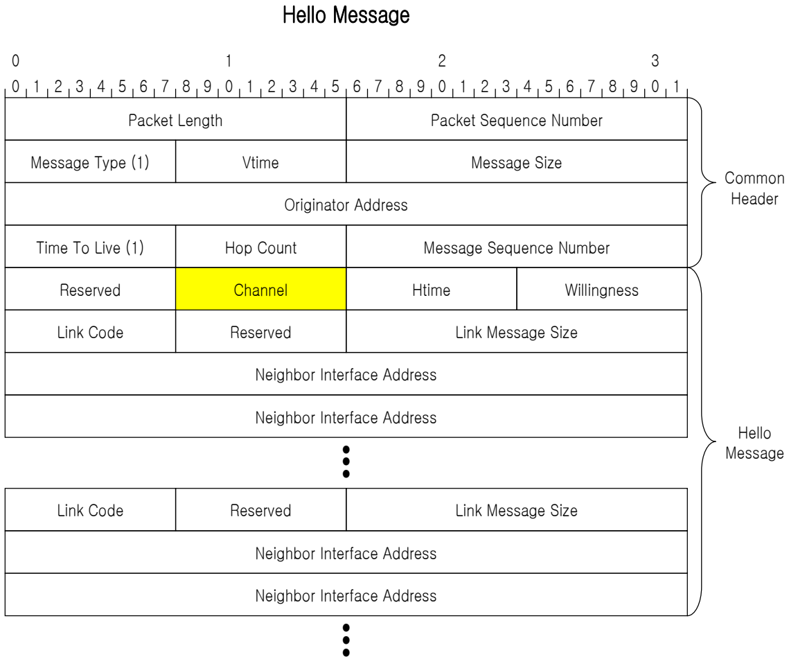
Figure 4.6: OLSR-MC HELLO message.
