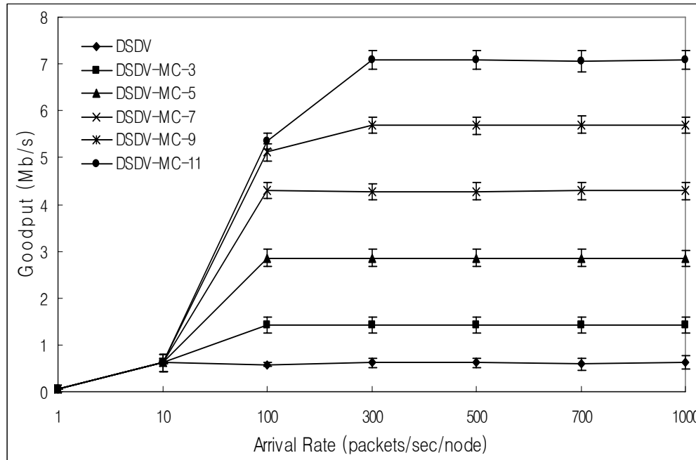
Figure 6.7: Goodput for single-hop network with varying packet arrival rate.
