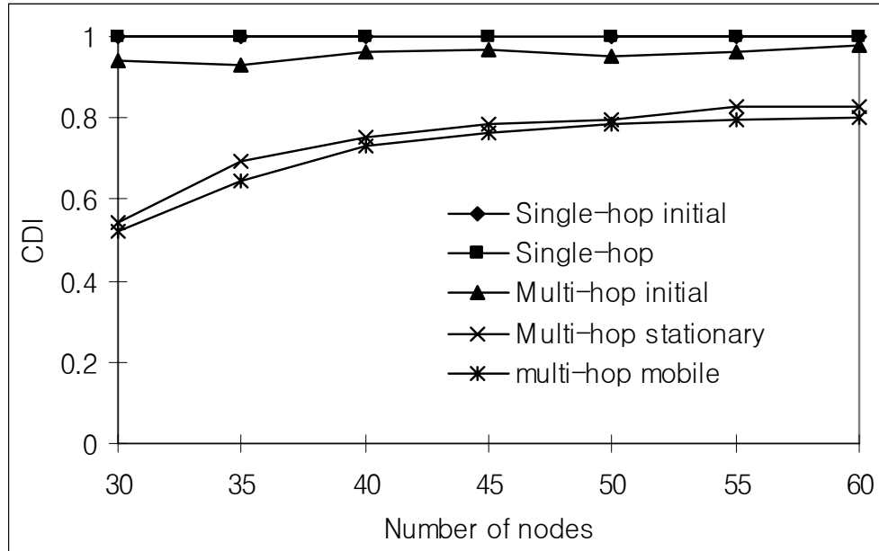
Figure 5.3: Channel distribution index after random exchanges.
