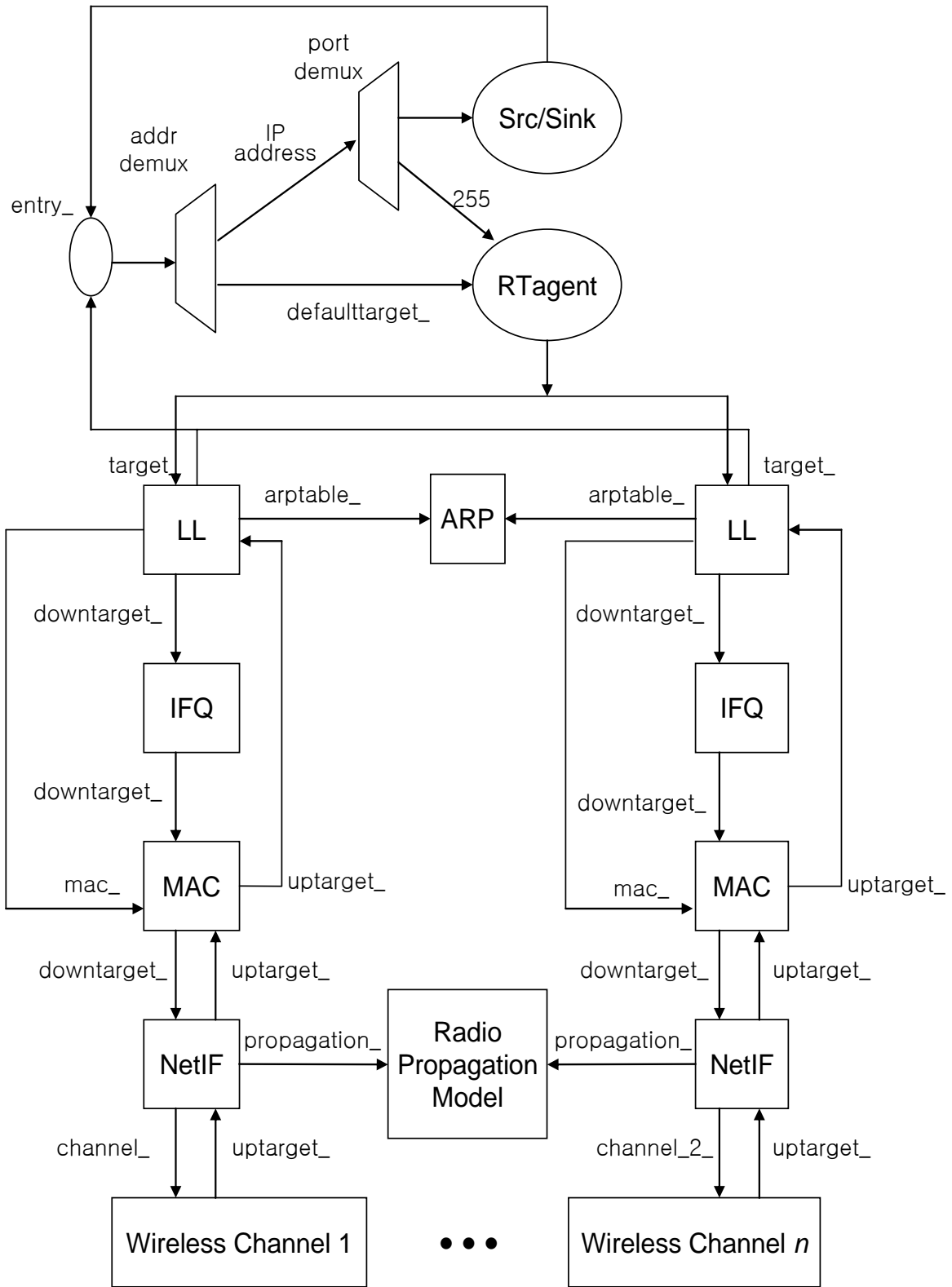
Figure 6.2: Schematic of the modified MobileNode object.
