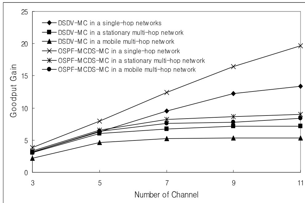
Figure 6.32: Goodput gain for varying numbers of channels.
