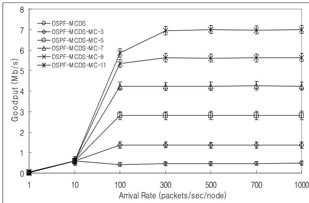
Figure 6.25: Goodput for single-hop network for varying packet arrival rate.
