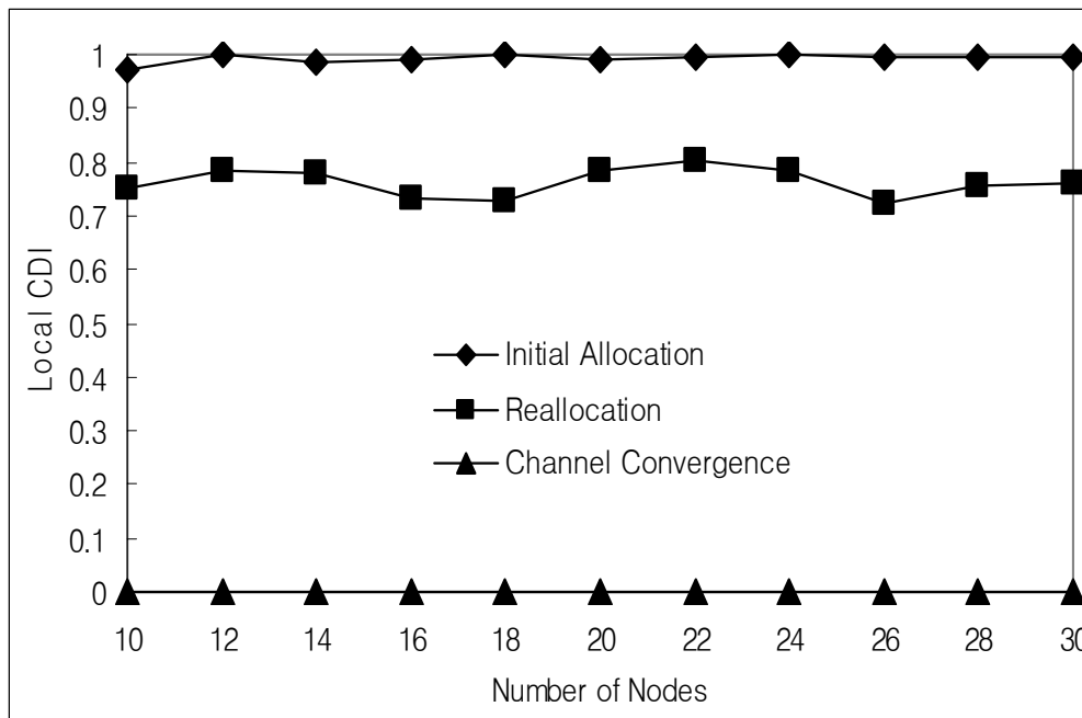
Figure 6.14: CDI for the single-hop network for varying numbers of nodes.
