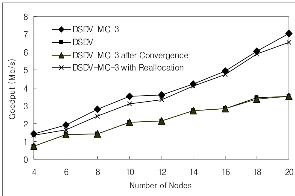
Figure 6.13: Goodput for linear network for varying numbers of nodes.
