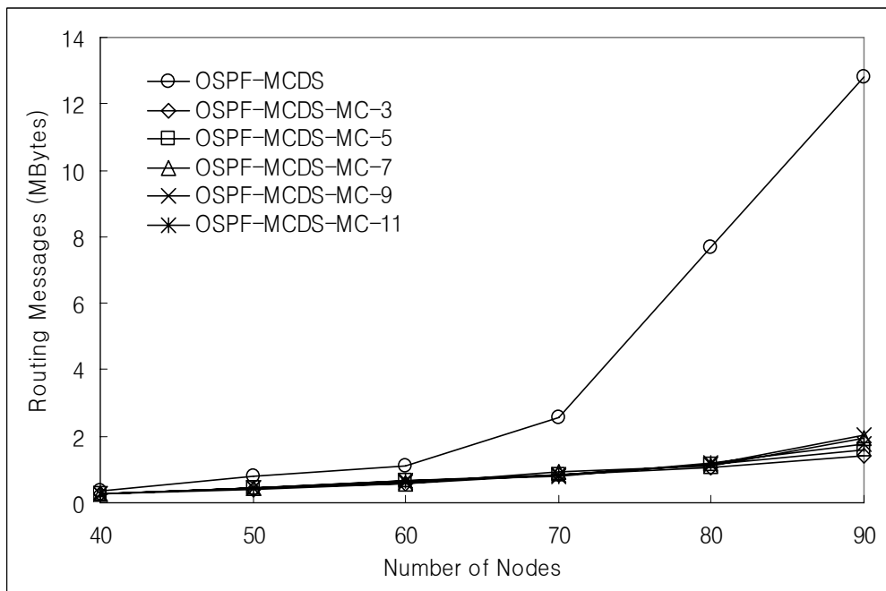
Figure 6.29: Number of routing messages for a mobile multiple-hop network for varying numbers of nodes.
