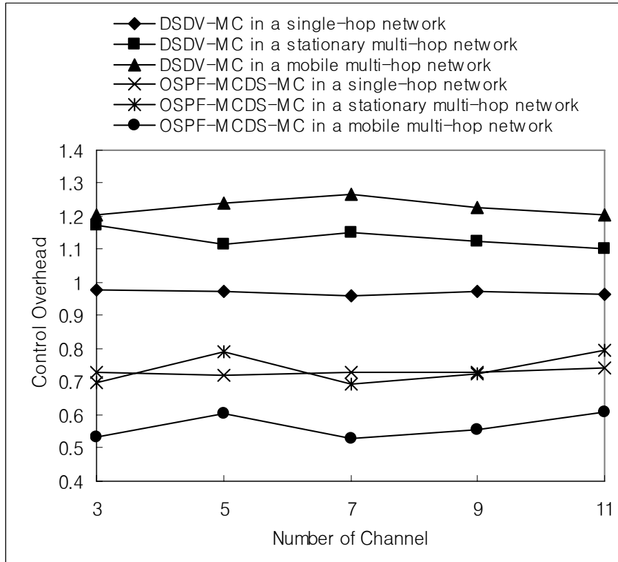
Figure 6.33: Control overhead for varying numbers of channels.
