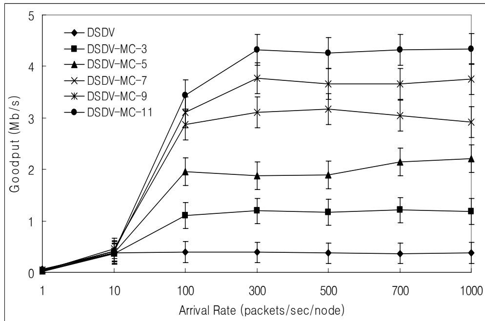
Figure 6.9: Goodput for varying packet arrival rates for a mobile multiple-hop network.
