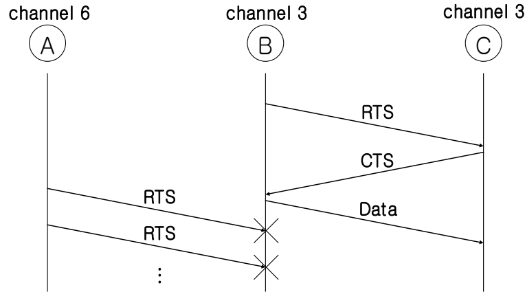
Figure 3.1: Channel synchronization problem.
