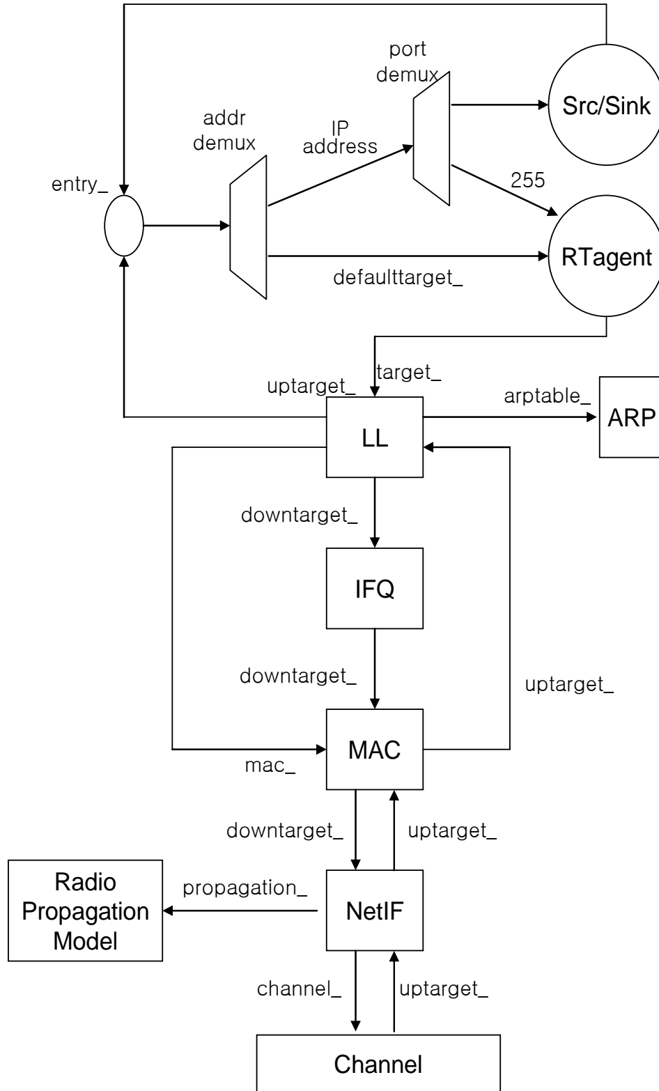
Figure 6.1: Schematic of a MobileNode object in ns2 [67].
