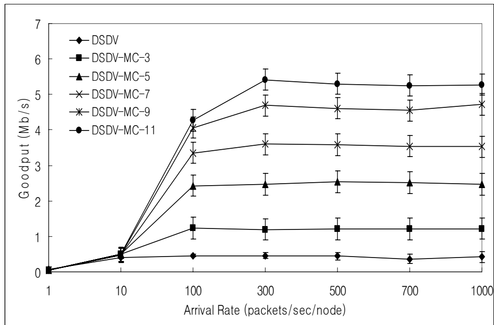
Figure 6.8: Goodput for varying packet arrival rates for a stationary multiple-hop network.
