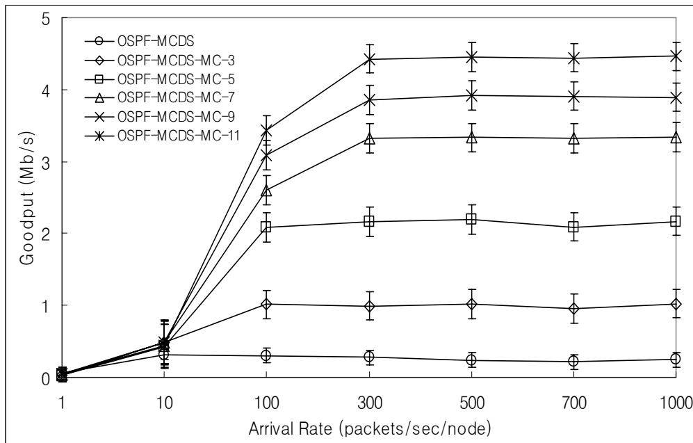
Figure 6.26: Goodput for stationary multiple-hop network for different packet arrival rates.
