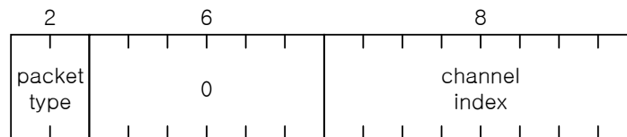
Figure 4.5: OSPF-MCDS-MC CU message.
