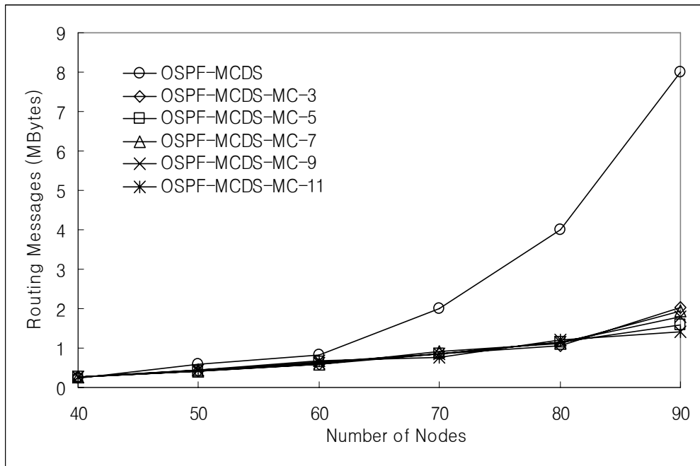
Figure 6.28: Number of routing messages for stationary multiple-hop network for varying numbers of nodes.
