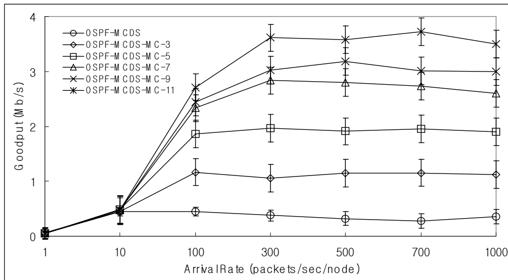
Figure 6.27: Goodput for mobile multiple-hop network for different packet arrival rates.
