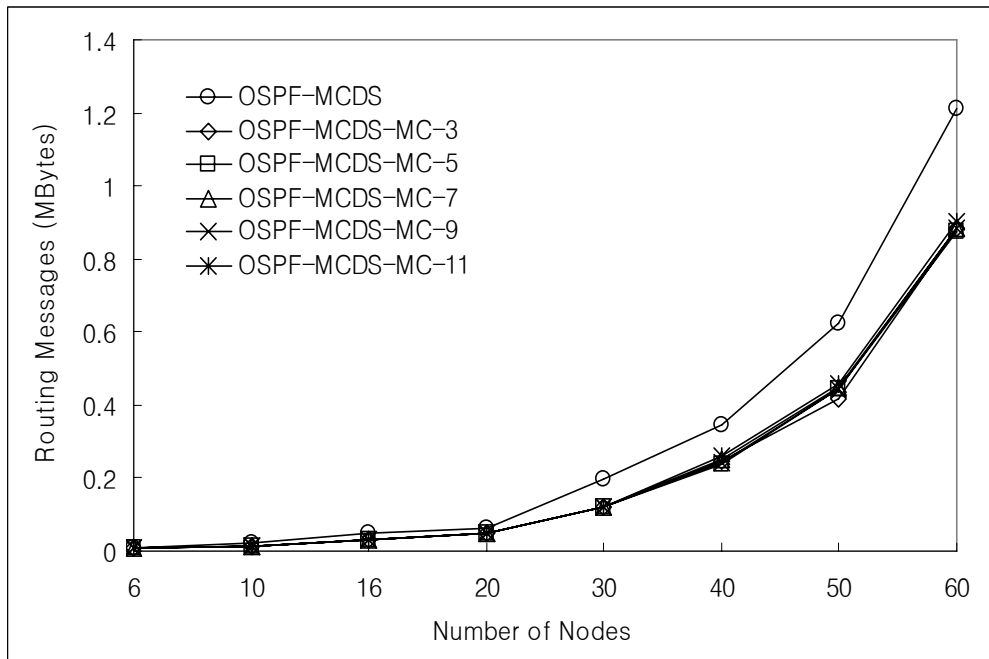
Figure 6.22: Routing messages for single-hop network for different numbers of channels and different numbers of nodes.
