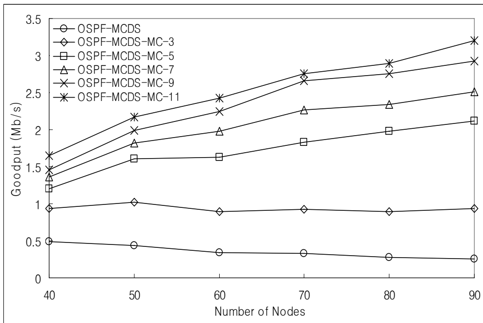
Figure 6.31: Goodput for mobile multiple-hop network for varying numbers of nodes.
