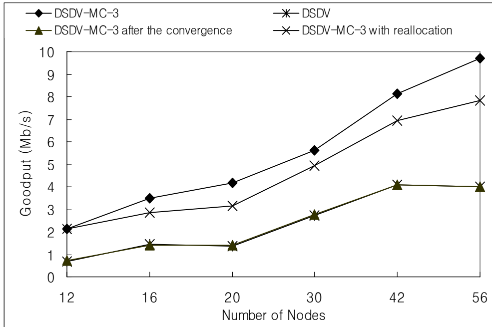
Figure 6.17: Goodput for multiple-hop network for varying numbers of nodes.
