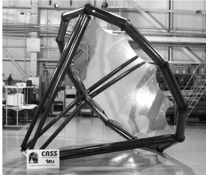
Figure 2.4: The inflatable hexapod structure for dynamic analysis. Photo courtesy of NASA / L. Horta.
