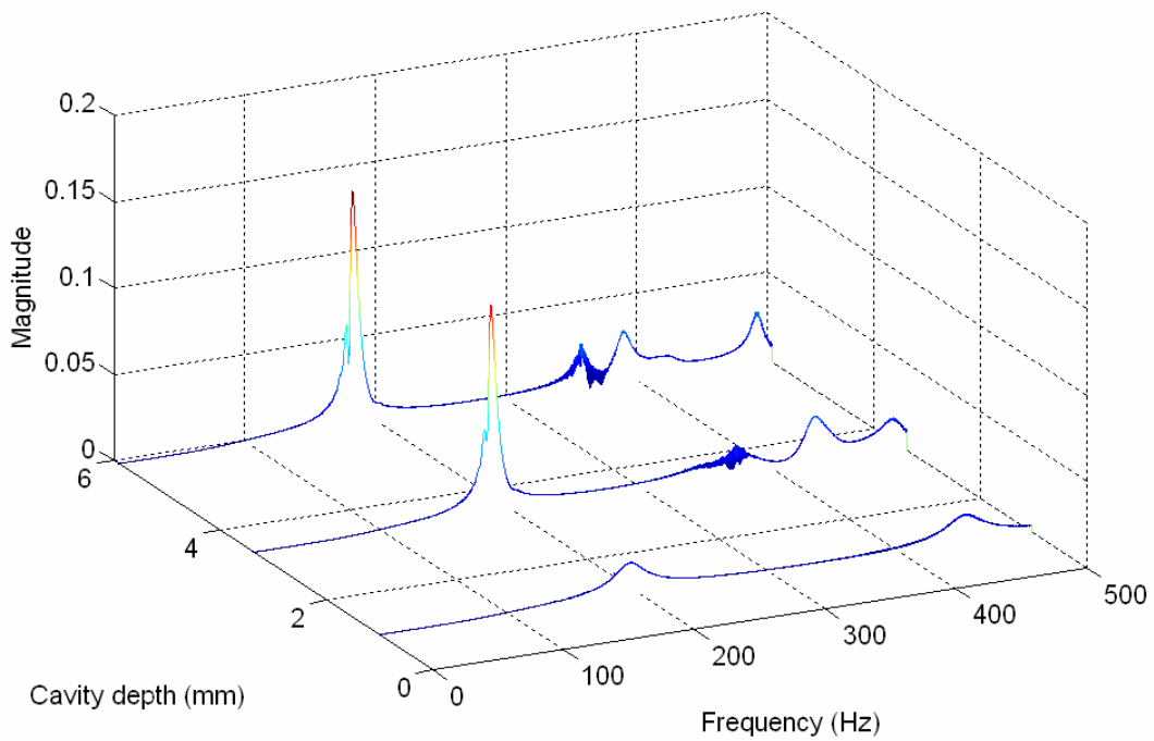
Figure 7.8. Frequency response function of the Mylar membrane at point 1 at 10 Torr. Note the enhanced, damped dynamics caused by the air-filled cavity.
