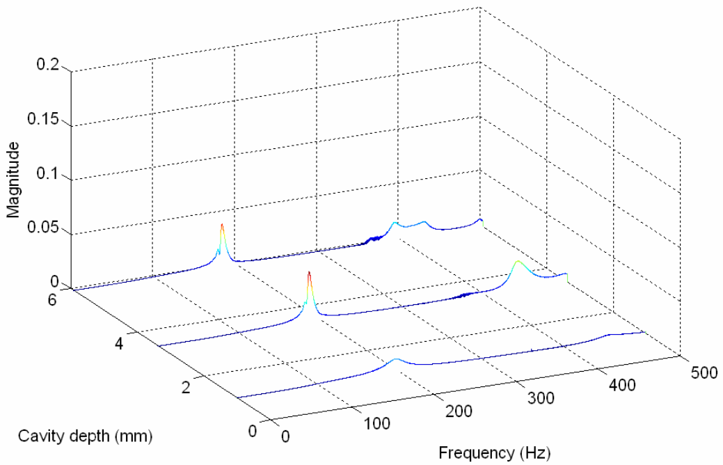
Figure 7.11. Frequency response function of the Mylar membrane at point 4 at 10 Torr. Note the enhanced, damped dynamics caused by the air-filled cavity.
