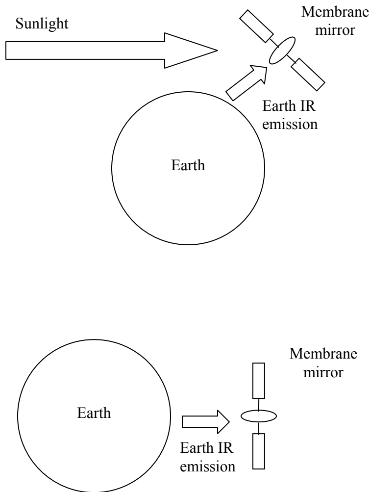
Figure 7.18. Extreme temperatures that the membrane mirror could encounter while on-orbit, from the hottest (top) to the coldest (bottom) cases.
