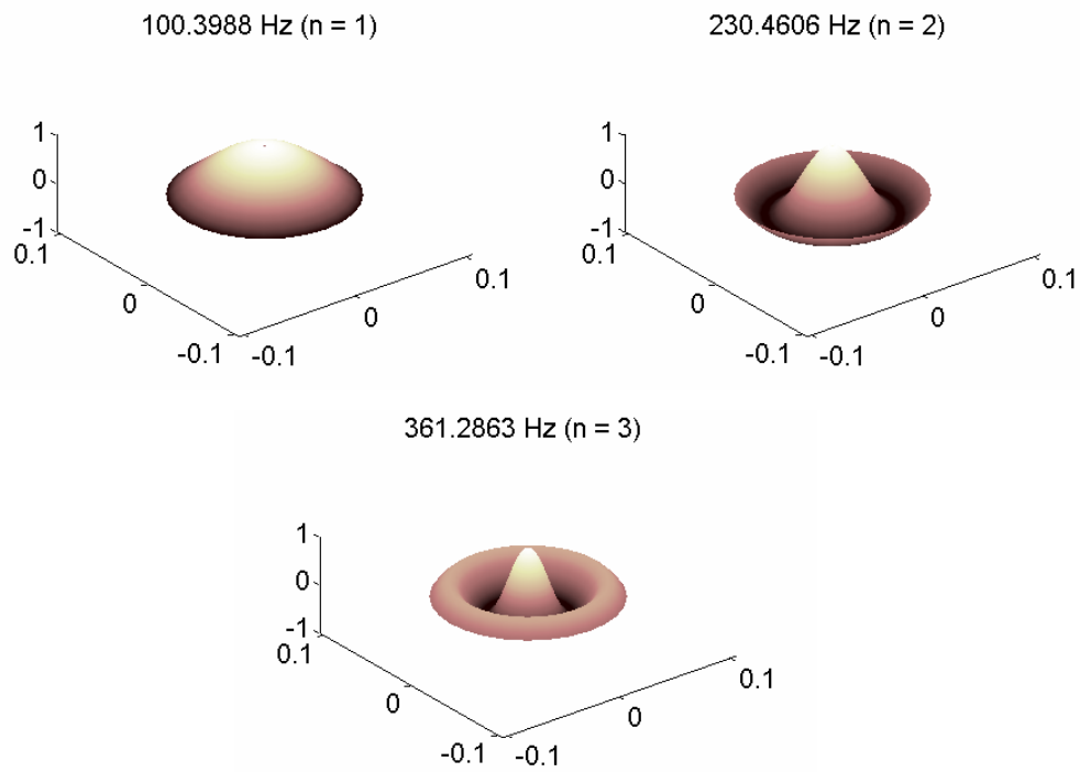
Figure 7.2. Mode shapes of an ideal membrane.
