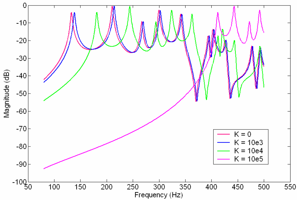
Figure 7.15. Simulated velocity response of a square membrane using different magnitudes for the stiffness value, K .
