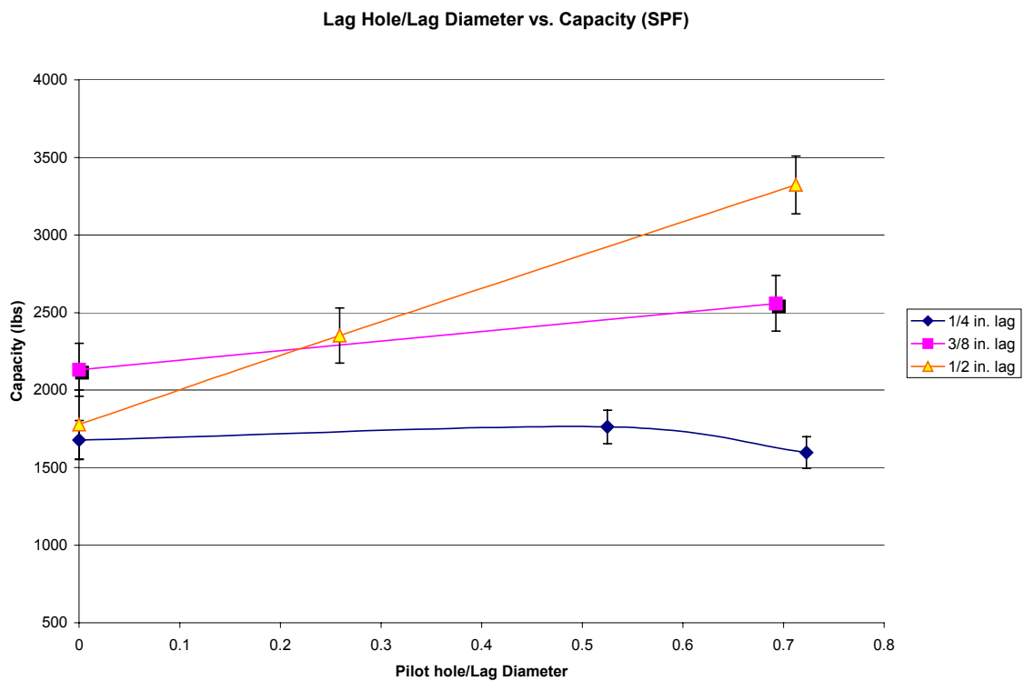
Figure H: Typical pilot hole / lag screw diameter vs. load graph (pilot hole vs. load is similar)
