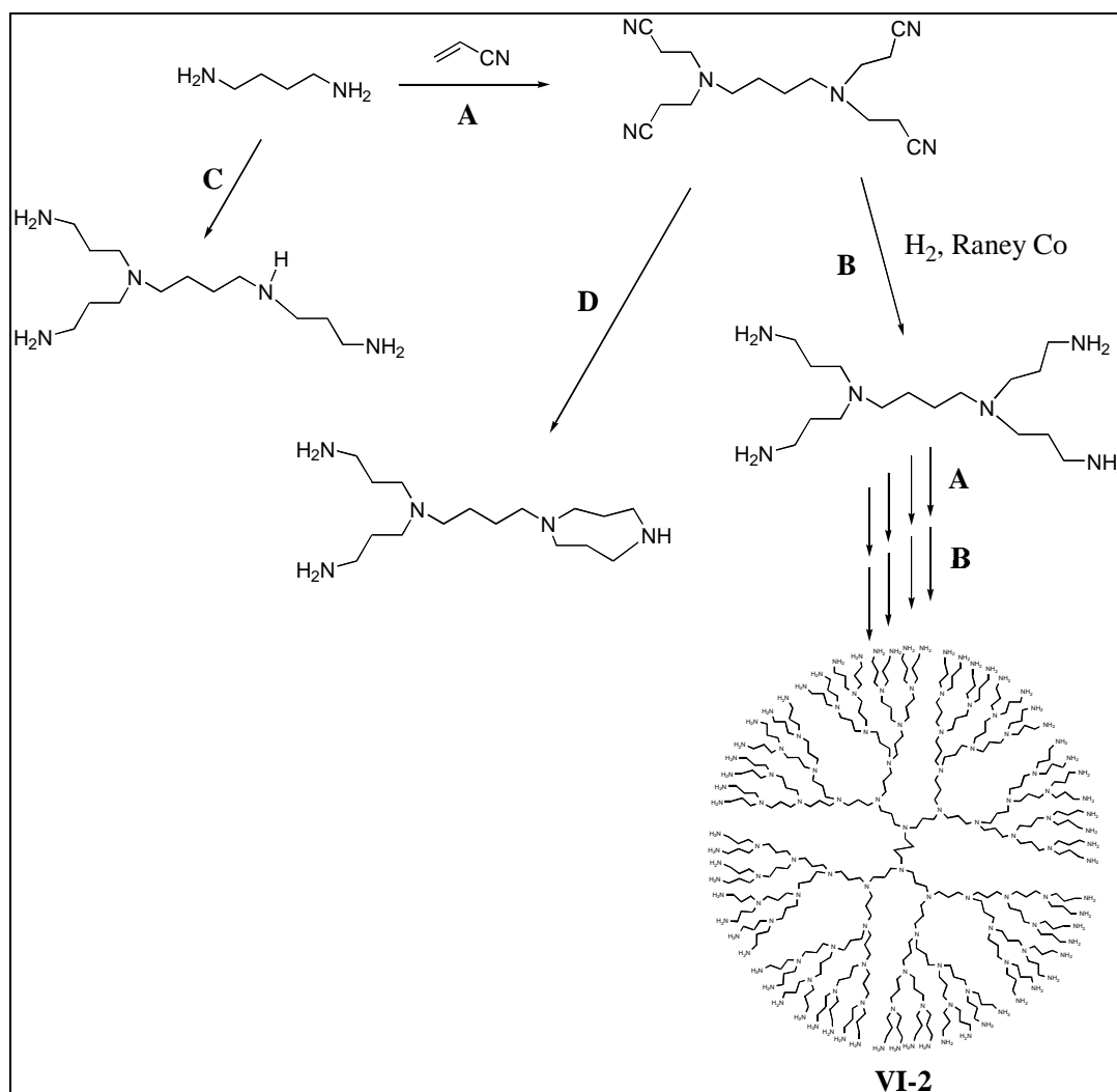
Figure VI-3. The synthesis of the poly(propylene imine) dendrimers (reactions A and B ) and alternative, unwanted reactions C and D as discussed in the text.
