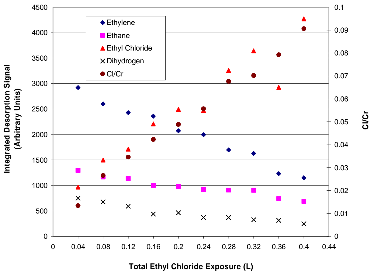
Figure 2.2 The relative desorbed quantities for each \text{CH}_3\text{-CH}_2\text{Cl} decomposition product, as well as the signal of the reactant molecule and Cl/Cr ratio, is shown above. The TDS experiment consisted of sequential 0.04 L doses over a nearly-stoichiometric \text{Cr}_2\text{O}_3 ( 10\bar{1}2 ) surface.
