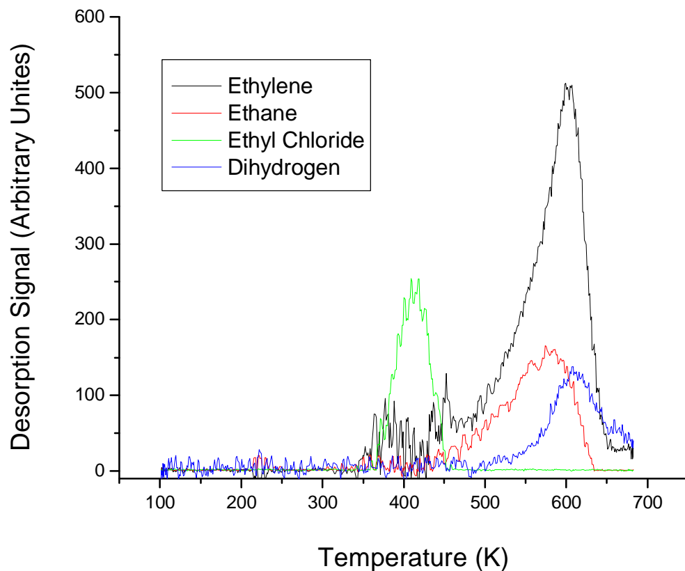
Figure 2.1 Desorption features observed following the first 0.04 L dose of \text{CH}_3\text{-CH}_2\text{Cl} in a TDS series. A desorption trace of the reactant ( \text{CH}_3\text{-CH}_2\text{Cl} ) is shown in green, the reaction products \text{CH}_2=\text{CH}_2 (black), \text{CH}_3\text{-CH}_3 (red) and \text{H}_2 (blue) are also shown.
