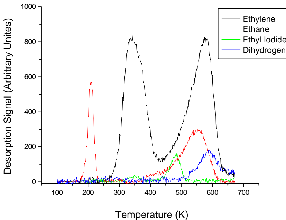
Figure 3.1 Desorption features observed following the first 0.04 L dose of \text{CH}_3\text{-CH}_2\text{I} on a clean, nearly-stoichiometric surface. A desorption trace of the reactant ( \text{CH}_3\text{-CH}_2\text{I} ) is shown in green (this trace is from the 5 th 0.04 L dose and enlarged 5 times), the reaction products \text{CH}_2=\text{CH}_2 (black), \text{CH}_3\text{-CH}_3 (red) and \text{H}_2 (blue) are also shown.
