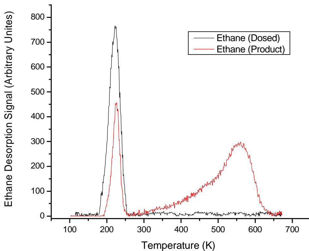
Figure 3.5 Comparison of TDS trace of \text{CH}_3\text{-CH}_3 product from the 2 nd dose 0.04 L ethyl iodide decomposition with the trace obtained from dosed ethane (0.02 L) on a nearly-stoichiometric \text{Cr}_2\text{O}_3 ( 10\bar{1}2 ) surface. The high temperature feature is absent from the dosed ethane trace.
