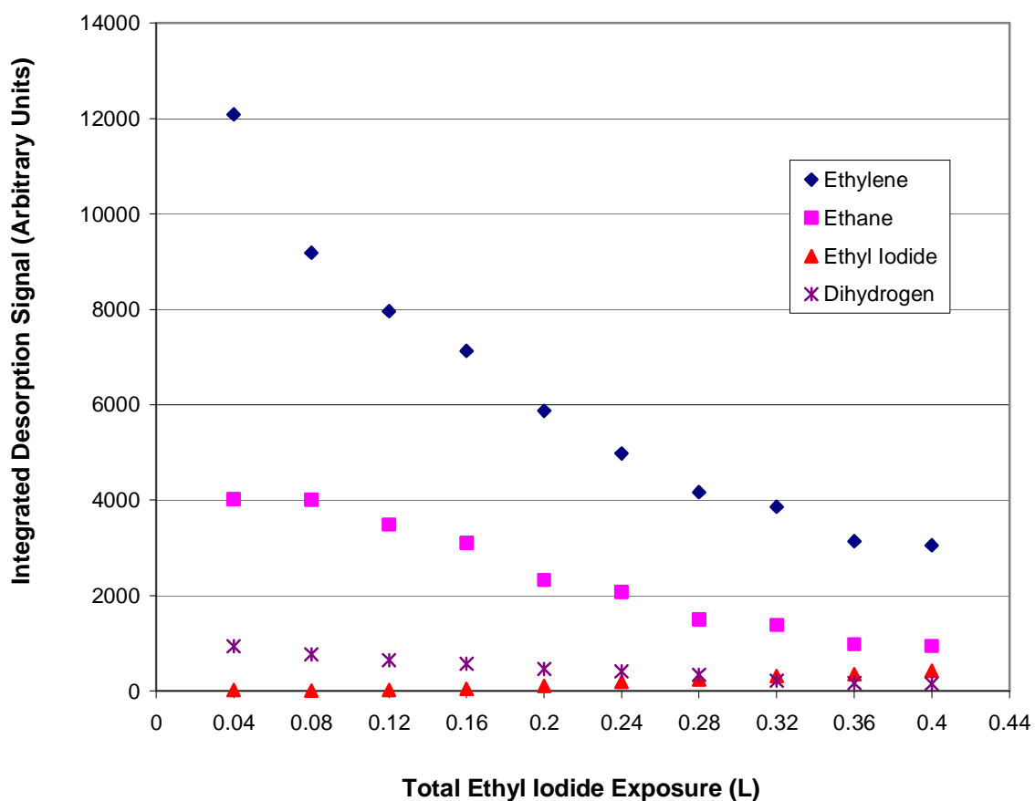
Figure 3.2 The relative quantities desorbed for each \text{CH}_3\text{-CH}_2\text{I} decomposition products, as well as the signal of the reactant molecule are shown above. The TDS experiment consisted of sequential 0.04 L doses over a nearly-stoichiometric \text{Cr}_2\text{O}_3 ( 10\bar{1}2 ) surface.
