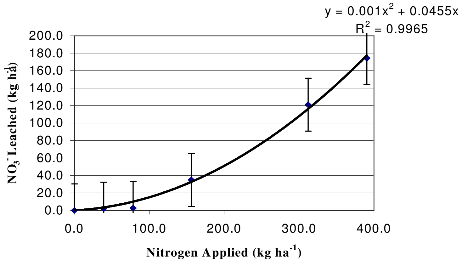
Figure 2.4 Total Applied Nitrogen Leached After the 1999 Bermudagrass Sprig Establishment Lysimeter Study in Blacksburg, VA.
