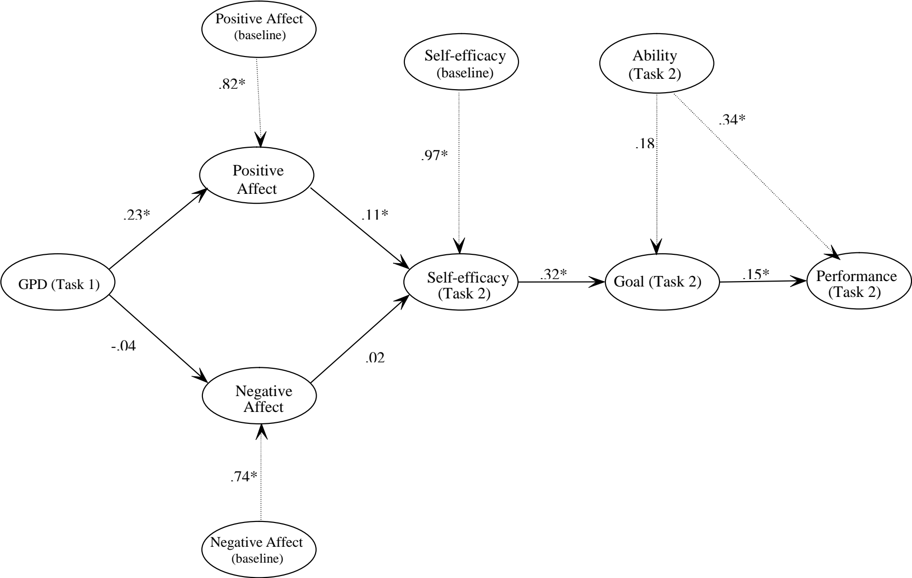
Figure 3. Proposed model with standardized path coefficients.
