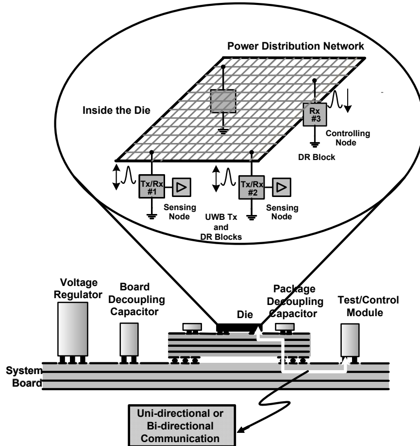
Figure 1.1: Power line communication in microprocessor environment.
