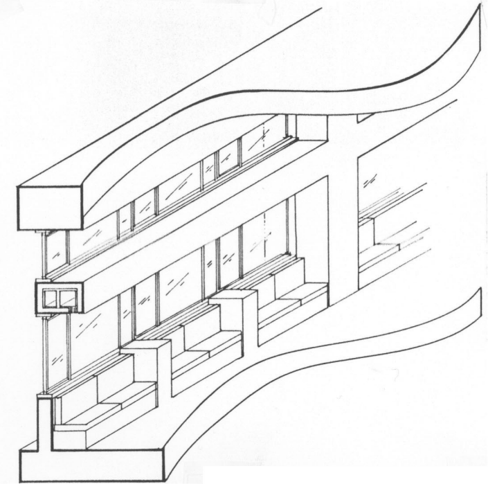
Cutaway axonometric of benches at classroom corridor.
