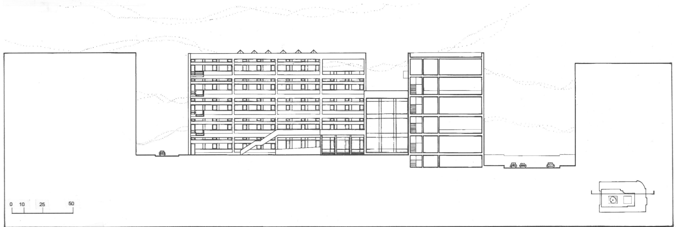
Courtyard elevation of classroom building.
