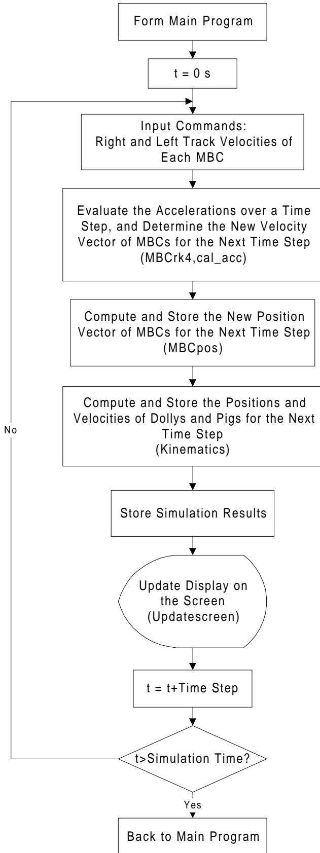
Figure B.2. Flowchart of the Simulation Module of the Two_MBC_Simulation Program Note: The function name that performs a task presents in a parenthesis
