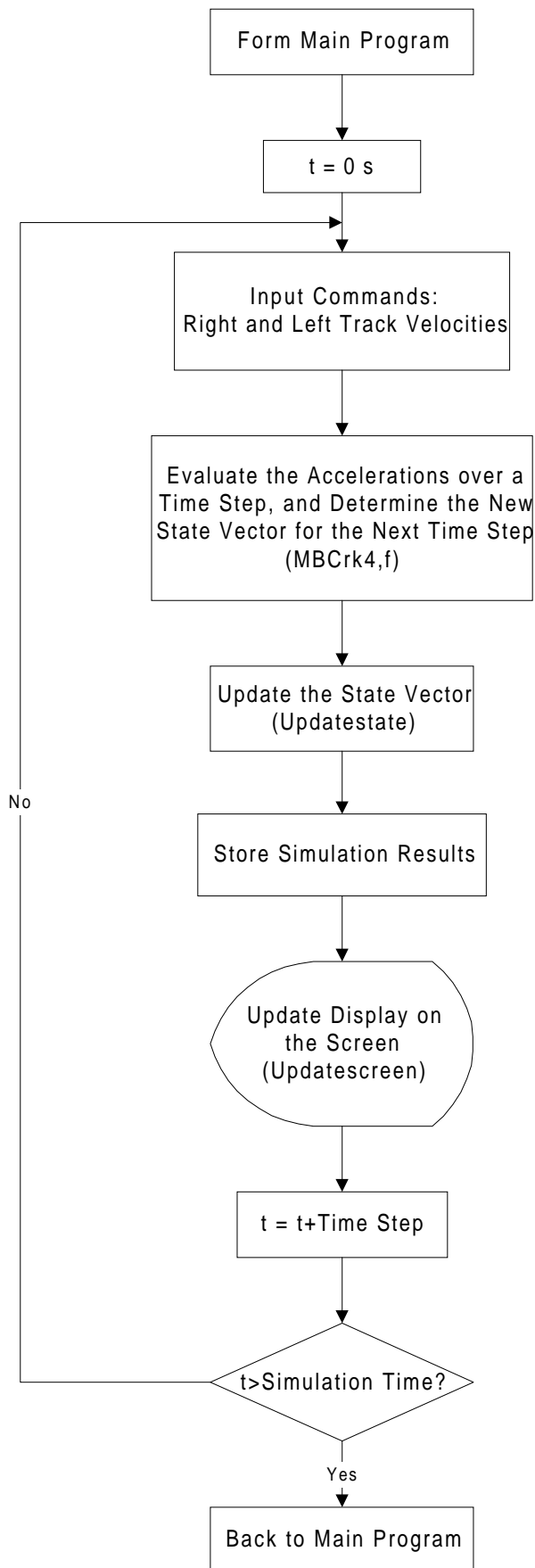
Figure A.2. Flowchart of the Simulation Module of the Single_MBC_Simulation Program
