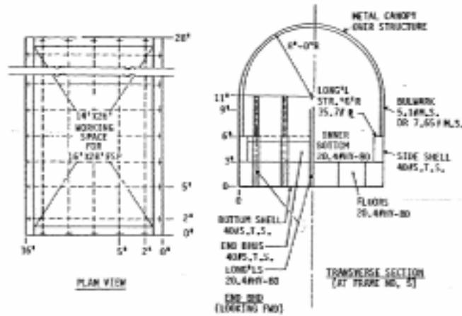
Figure 4.6: Floating Shock Platform
