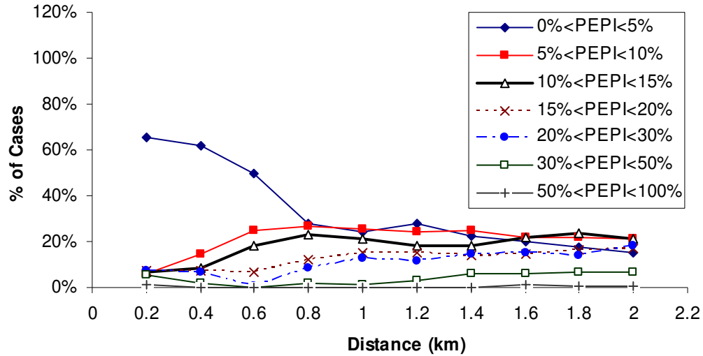
Figure 6.9: Percent of cases having different percent of extra P.I. for Robertson's model.
