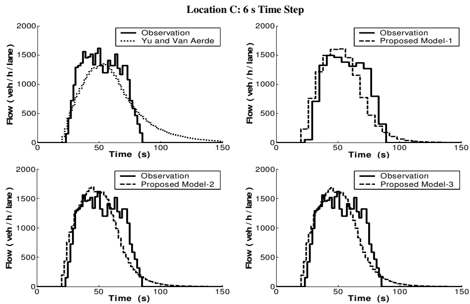
Figure 4.4: Observed and predicted downstream flow profiles (Montréal Data).
