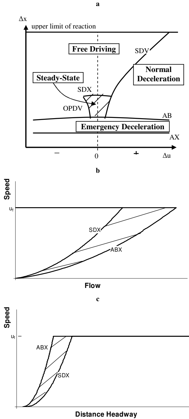
Figure 7.3: VISSIM's car-following model a. thresholds and regimes, b & c. steady-state behaviour.
