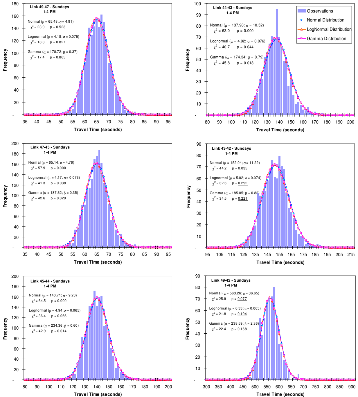
Figure 6.1: Observed distributions of travel times on I-35 South.
