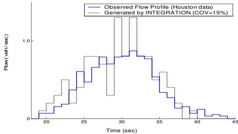
Figure 6.3: Observed and simulated flow profiles for Houston data.
