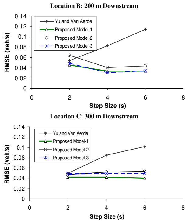
Figure 4.5: Error in predicted downstream flow profile.
