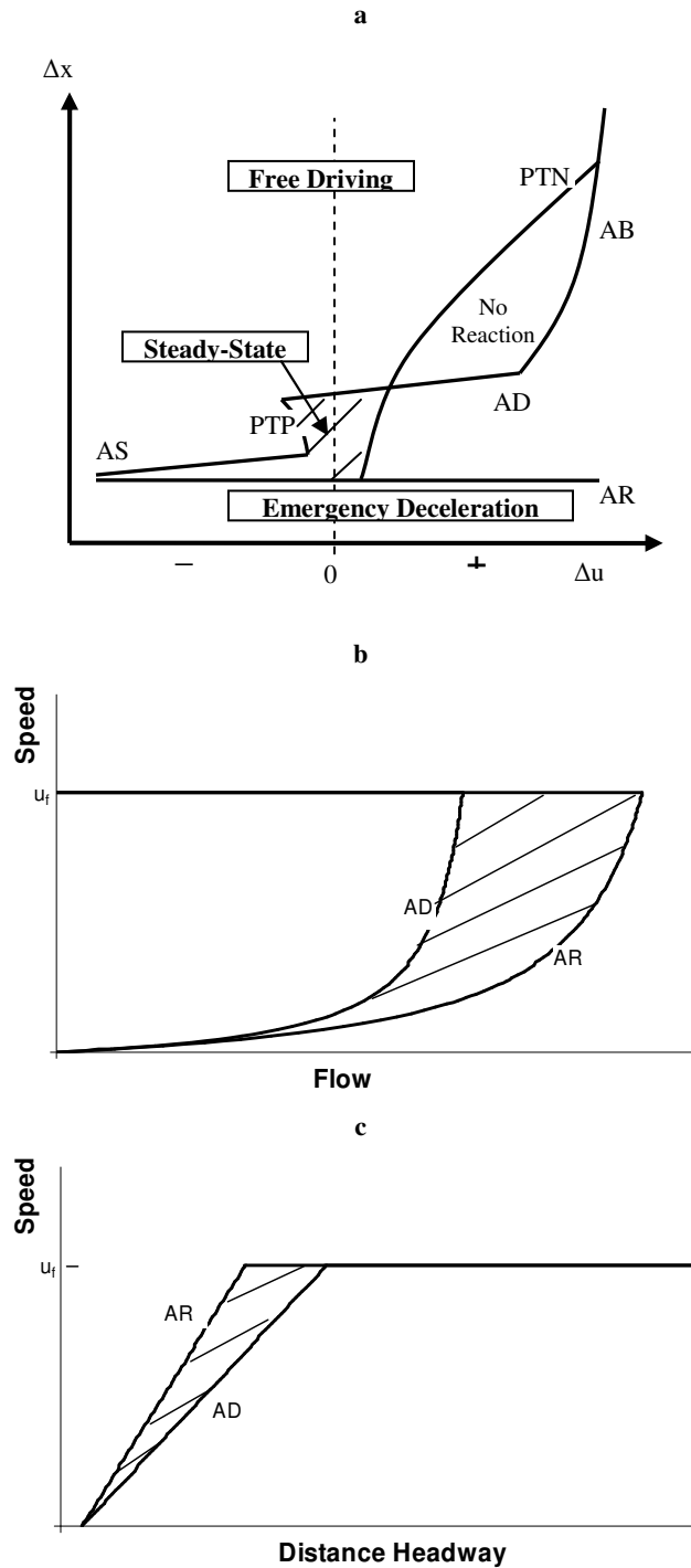
Figure 7.4: Fritzsche's car-following model a. thresholds and regimes, b & c. steady-state behaviour.
