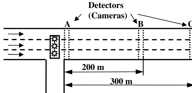
Figure 4.3: Montreal field test site and simulated network configuration.
