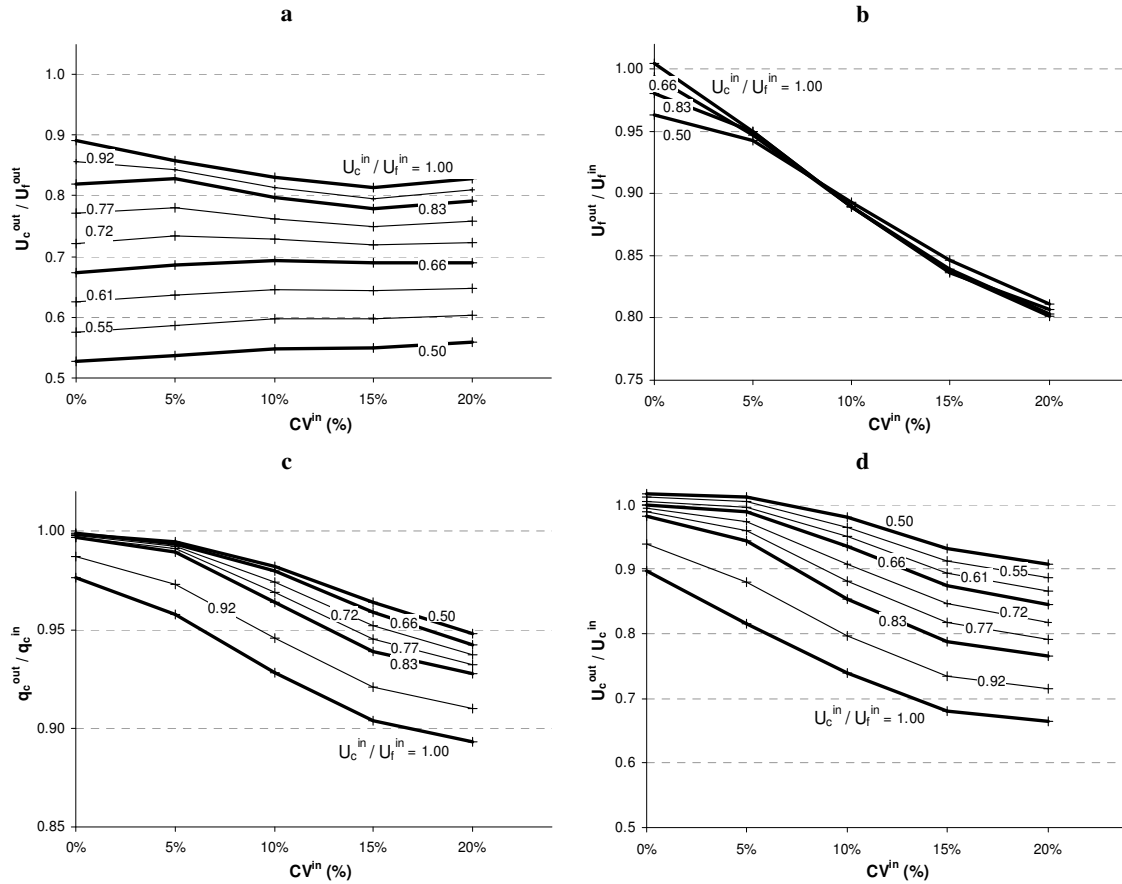
Figure 7.7: Effect of speed variability on the steady-state parameters.
