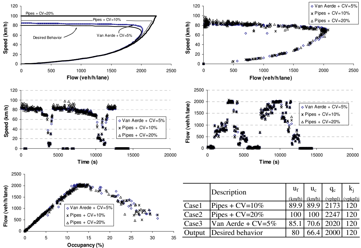
Figure 7.8: Application example of the proposed method.
