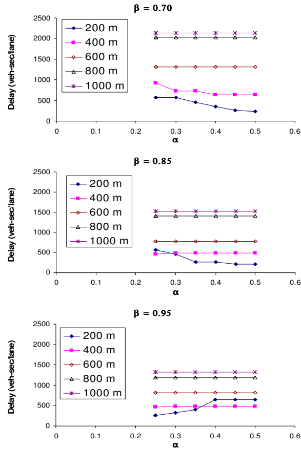
Figure 5.3: Variation of PI as function of platoon dispersion factor using 6-second step size (first case).
