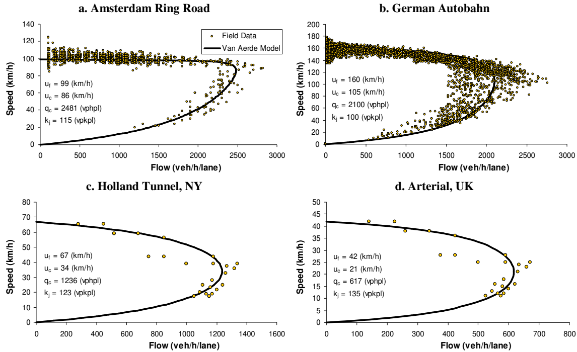
Figure 7.5: Field data and fitted Van Aerde model.
