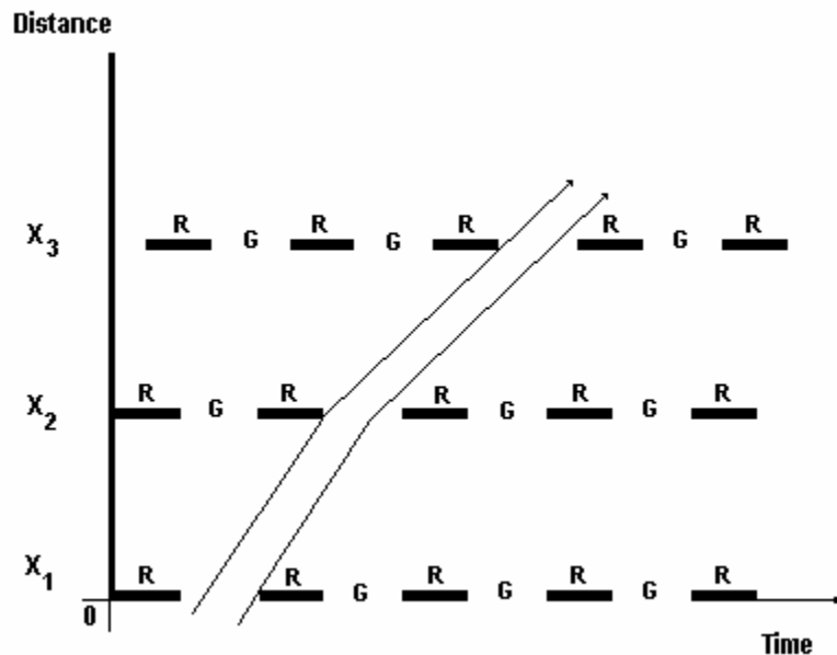
Figure 2.1: Space-time diagram for three intersections.
