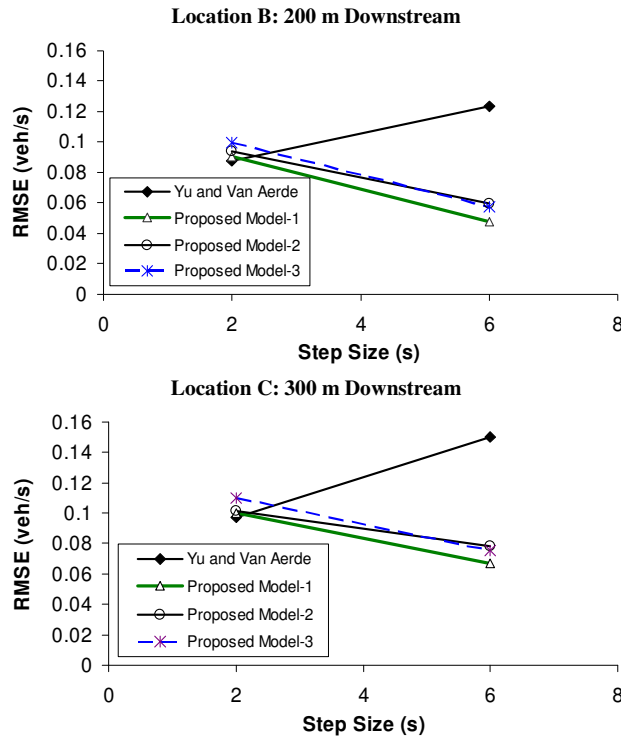
Figure 4.8: Error in predicted downstream flow profiles.
