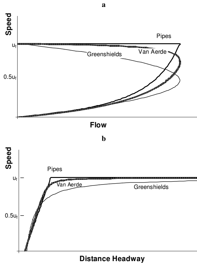
Figure 7.1: Steady state behaviours of Pipes, Greenshields, and Van Aerde models.
