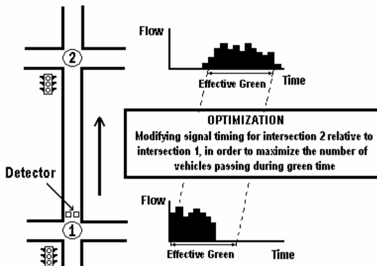
Figure 1.1: Platoon dispersion on an arterial and optimization of signal timing.
