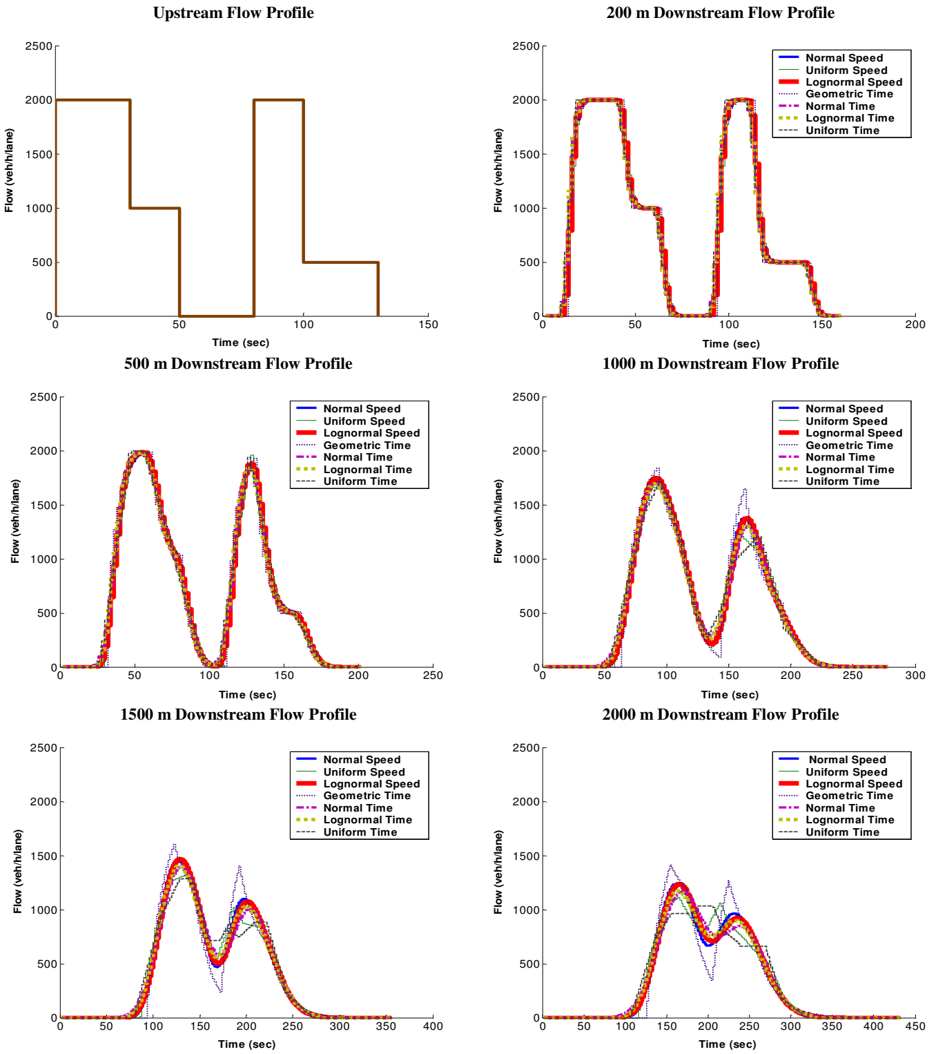
Figure 6.4: Upstream and predicted downstream flow profiles.
