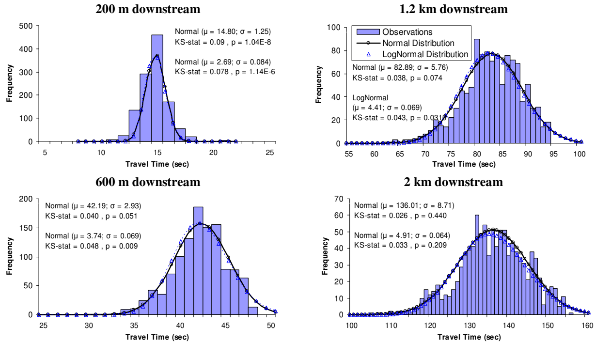
Figure 6.2: INTEGRATION results' distributions of travel times.
