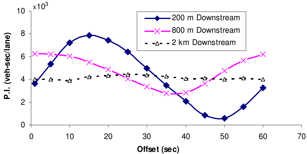
Figure 6.10: Offset-delay relationship for virtual signals at different distances.
