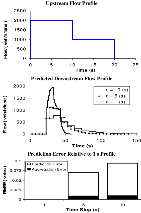
Figure 4.1: Upstream and predicted downstream flow profiles.
