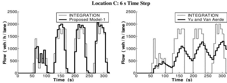
Figure 4.7: Simulated and predicted flow profiles.
