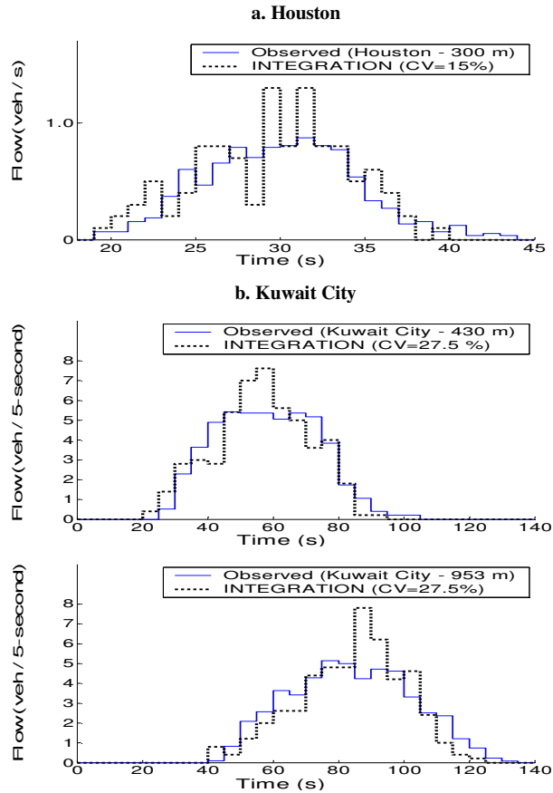
Figure 4.6: Observed and simulated downstream average flow profiles.
