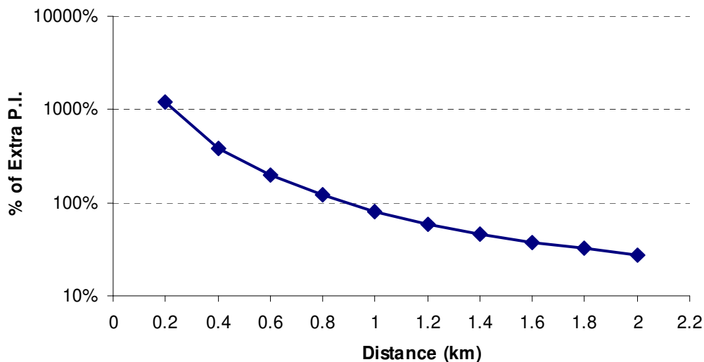
Figure 6.11: Average reduction in P.I. moving from random offsets to full coordination (%).
