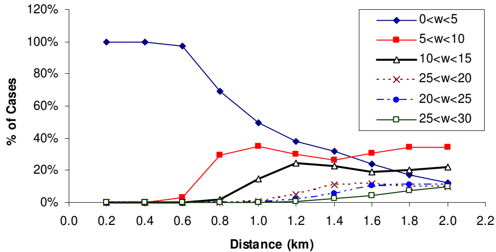
Figure 6.8: Percent of cases having different offset deviation ( w ) for Robertson's model.
