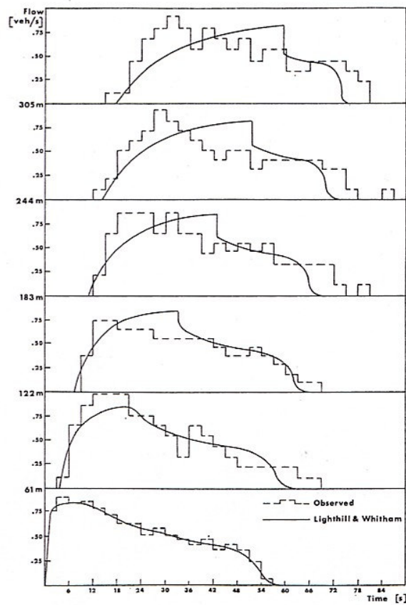
Figure 2.3: Observed flow patterns with those predicted by Lighthill and Whitham (Seddon, 1971).
