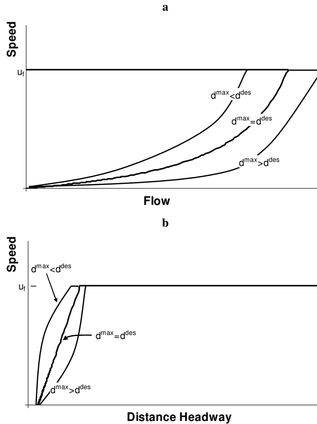
Figure 7.2: Steady-state behaviour of the Gipps model.
