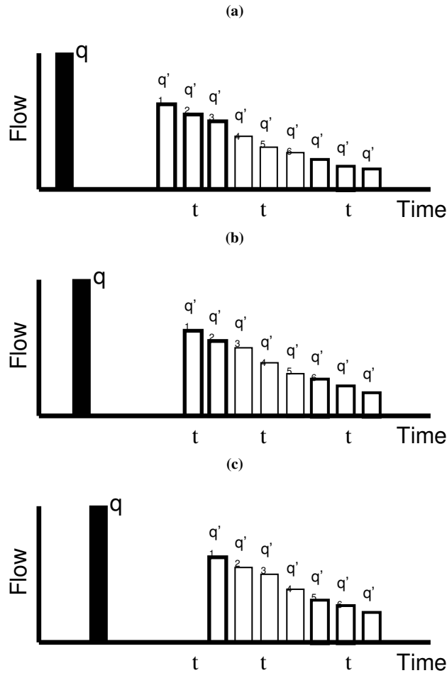
Figure 4.2: Parametric second-by-second platoon dispersion derivation.
