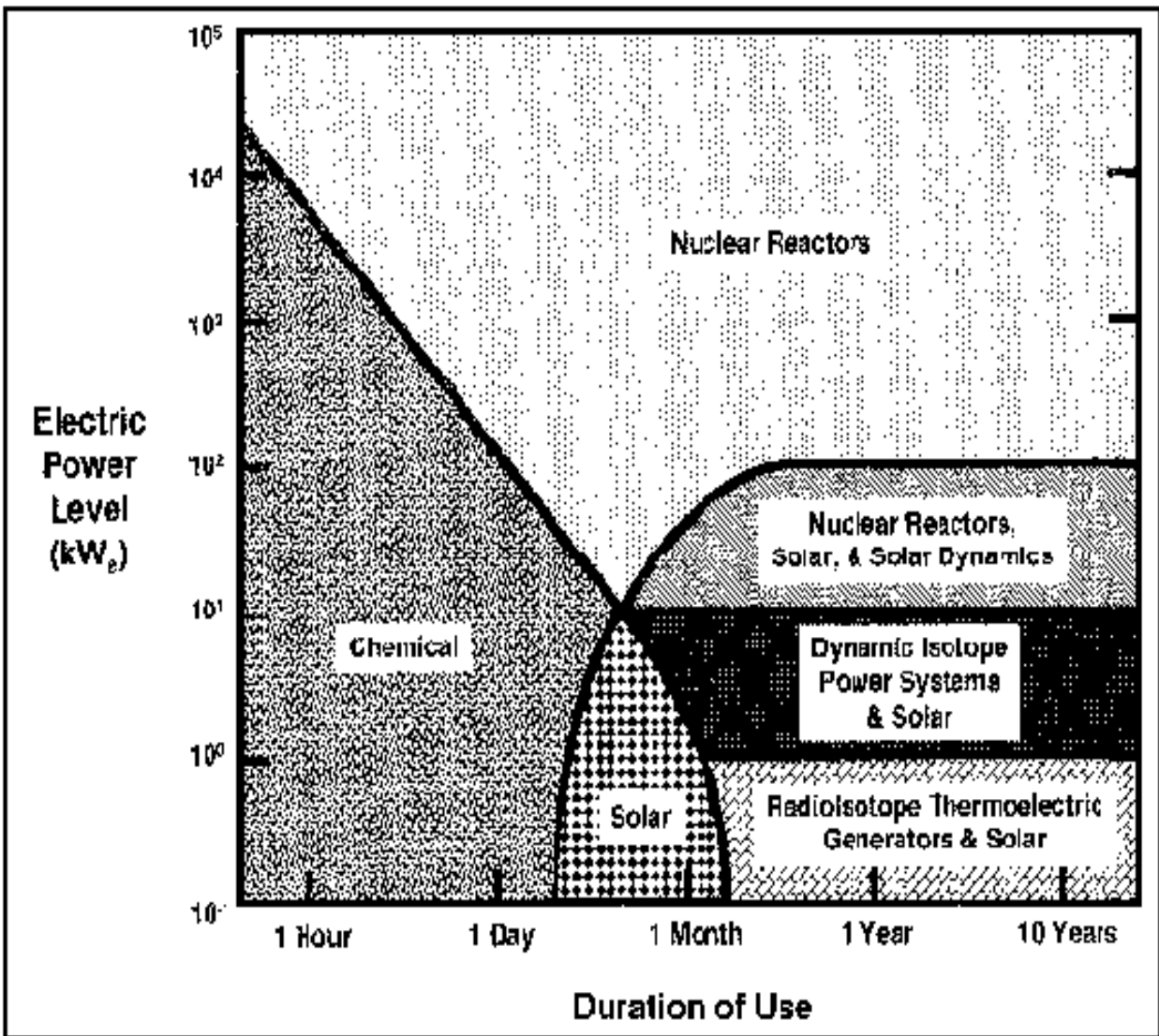
Figure 2 Comparisons of Space Power Systems
