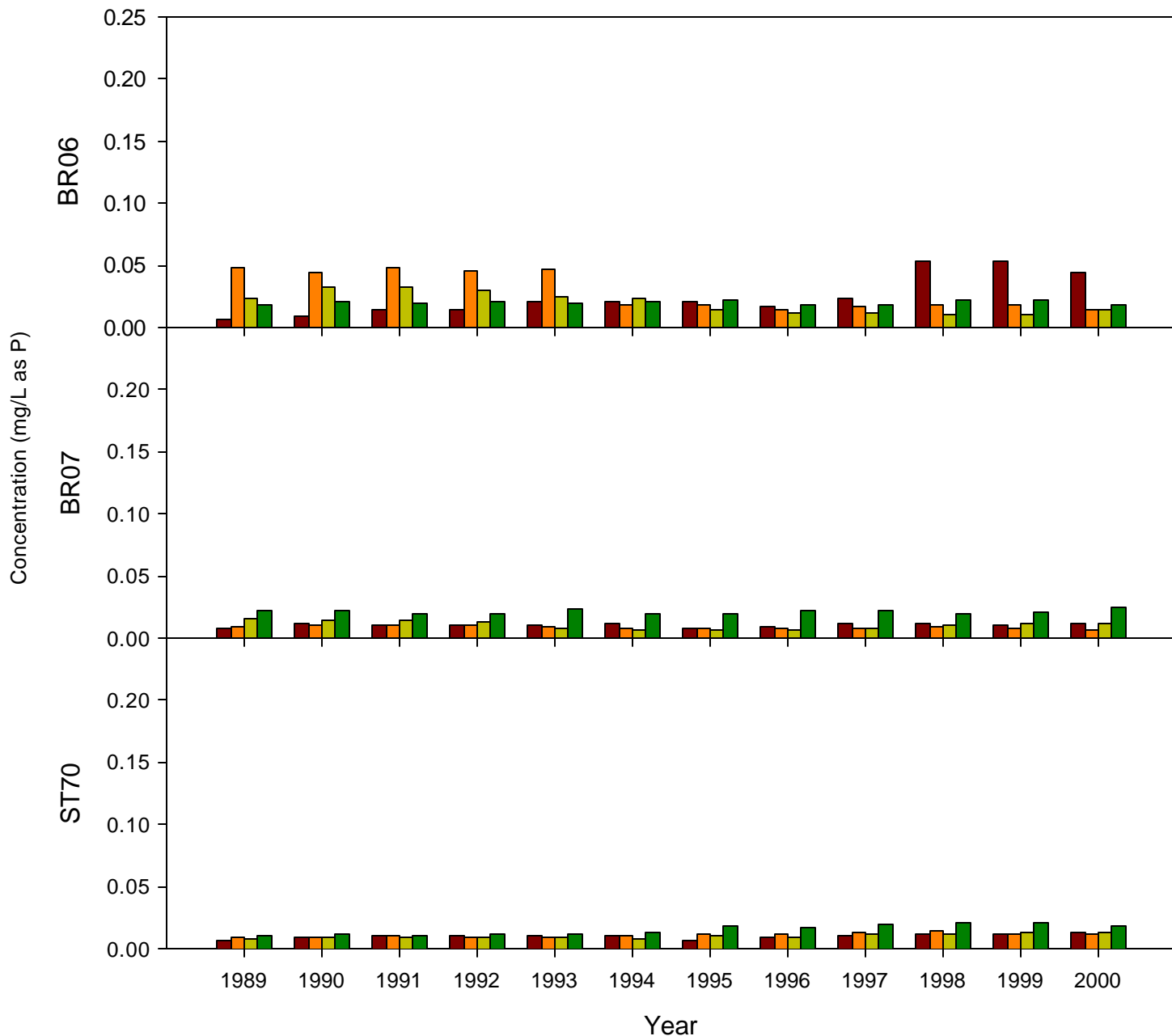
Figure 24 Lake Manassas Stream Stations Total Phosphorus 5 year running average
