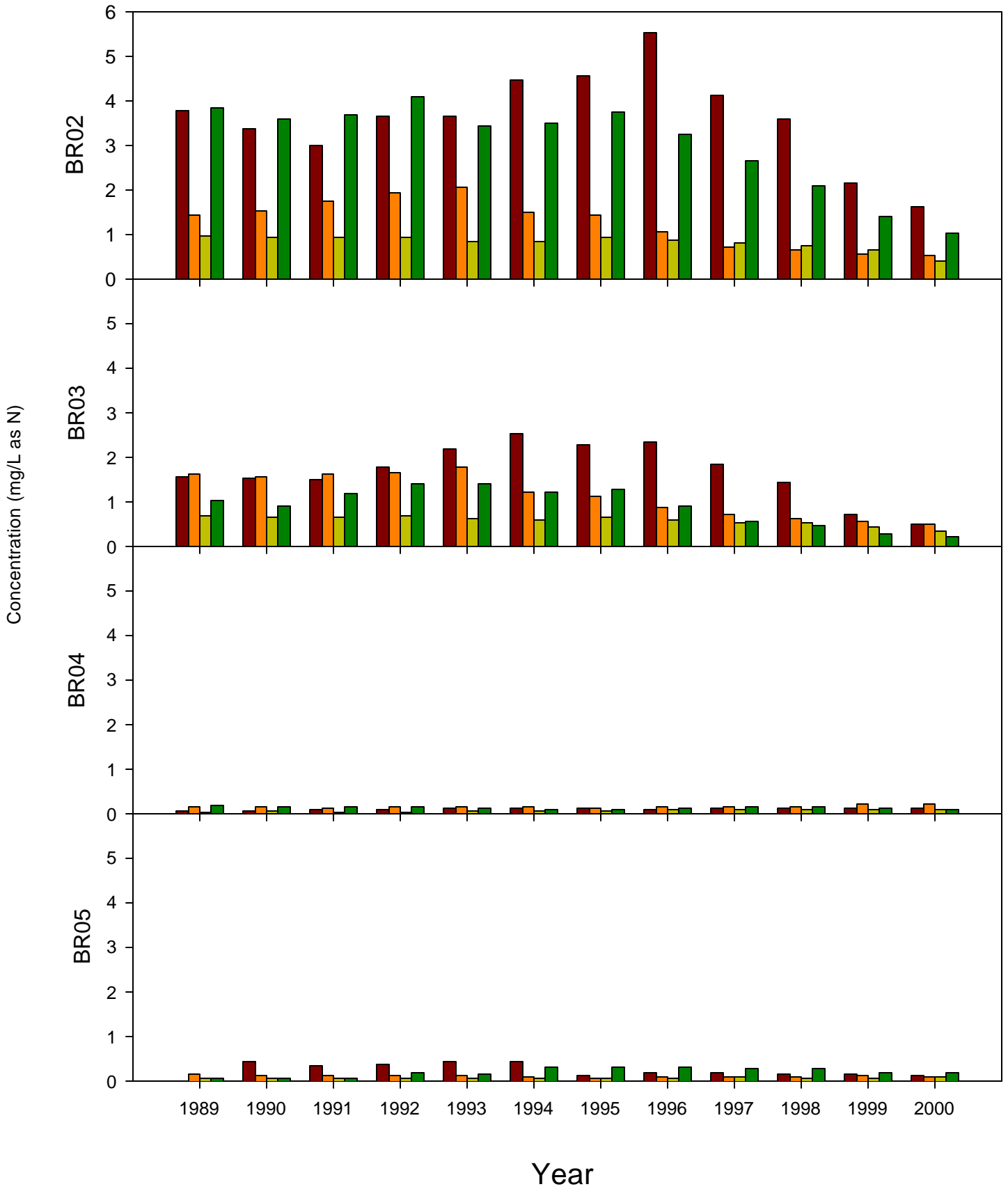
Figure 15 Lake Manassas Stream Stations Ox-N Concentration 5 Year Running Average
