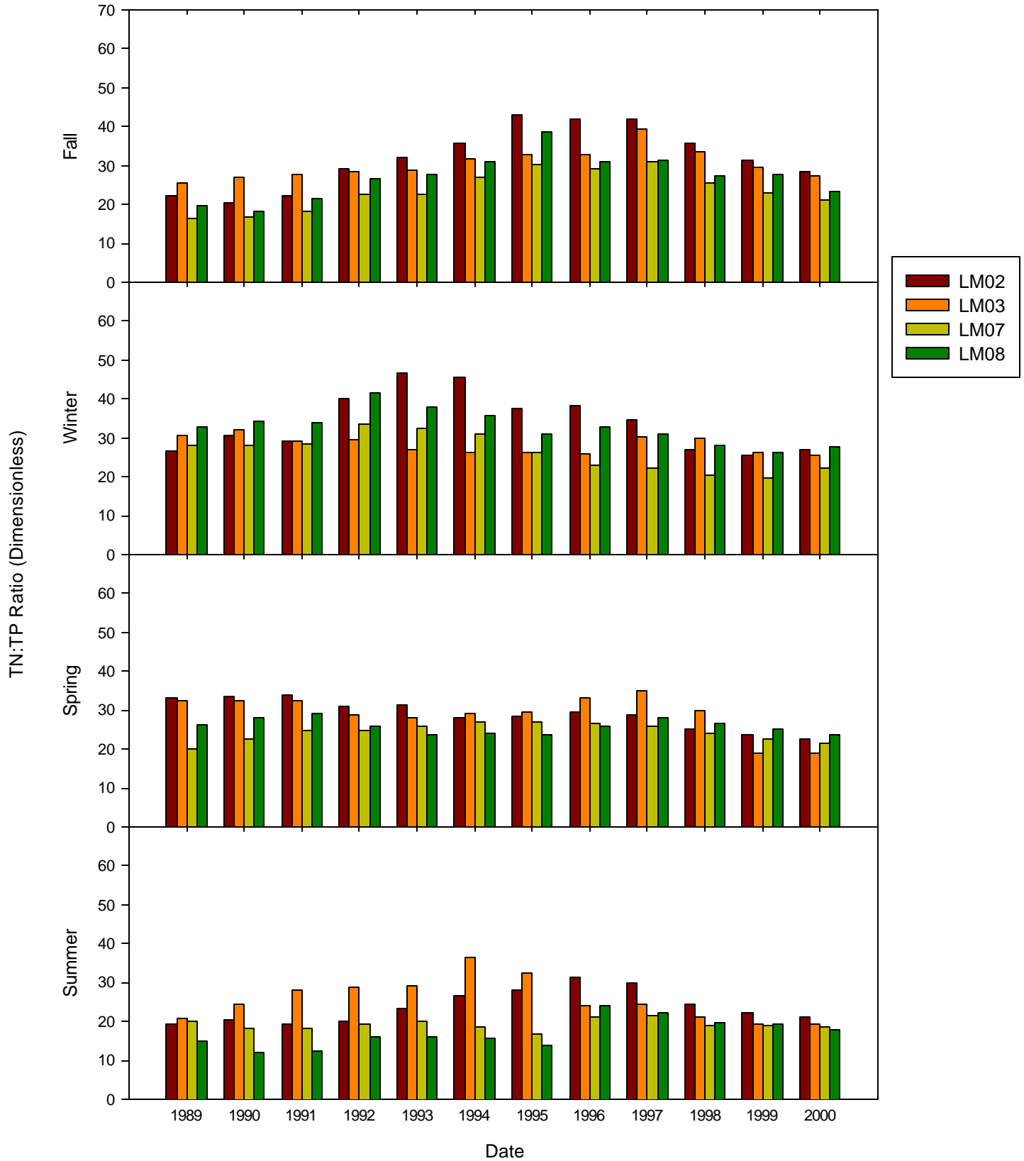
Figure 87 Lake Manassas (Surface) Seasonal 5 year Rolling Average TN:TP Ratios, 1984-2000
