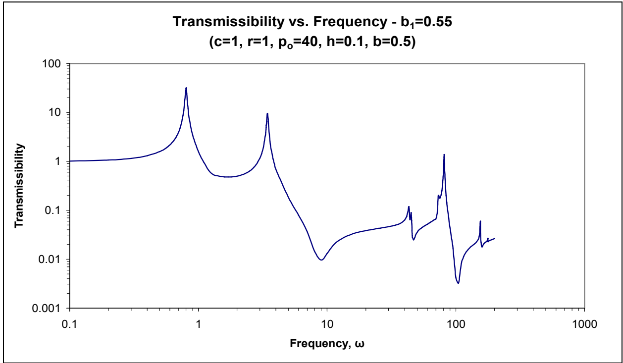
Figure E.1 Transmissibility vs. Frequency for b_1=0.55
