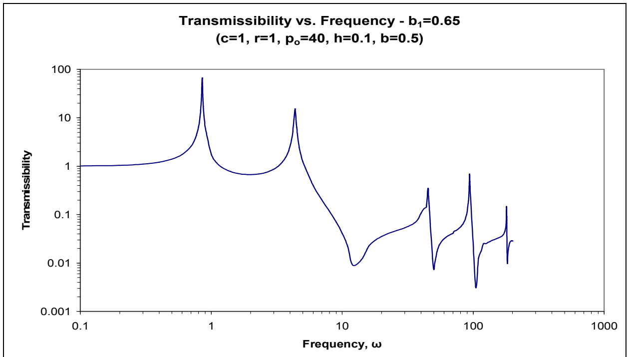
Figure E.2 Transmissibility vs. Frequency for b_1=0.65
