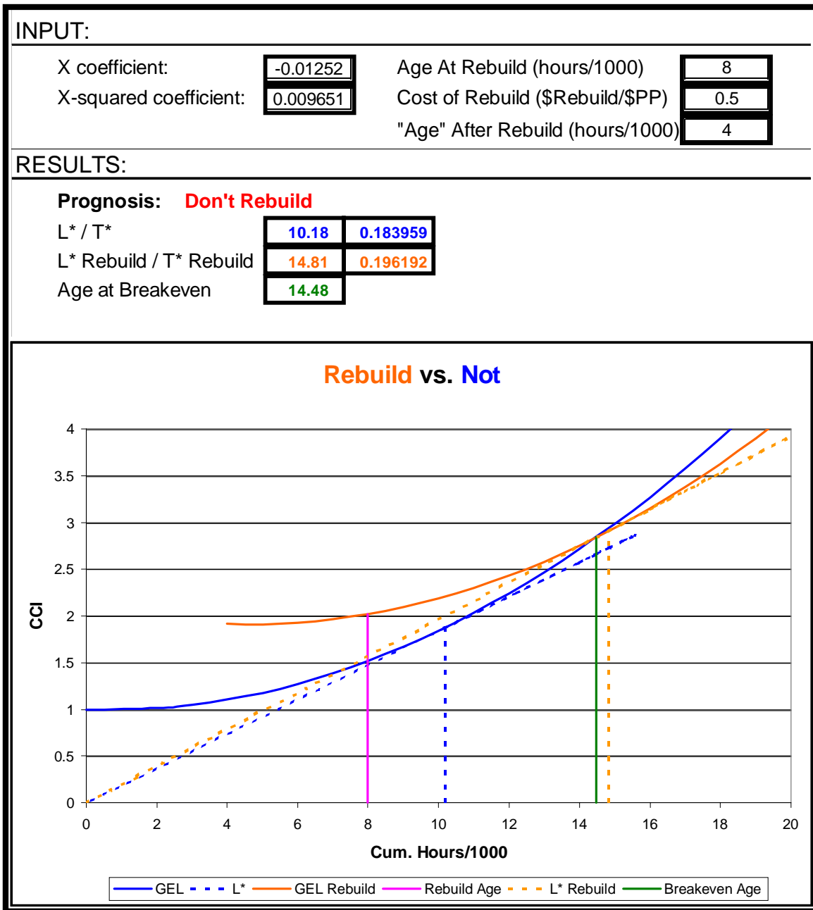
Figure 9-2: Rebuild Spreadsheet
