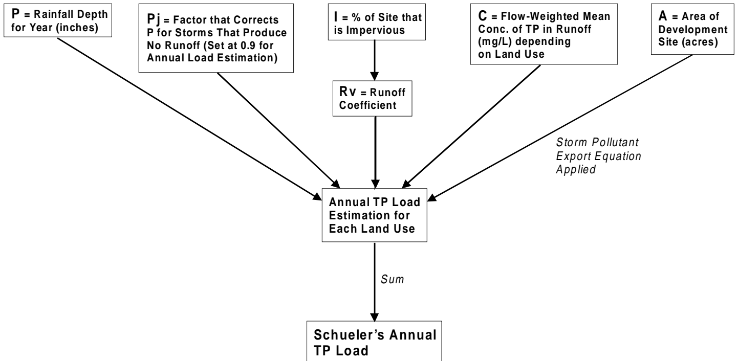
Figure A-4. Schematic of Schueler's Simple Method (1987) for TP Load Estimation.
