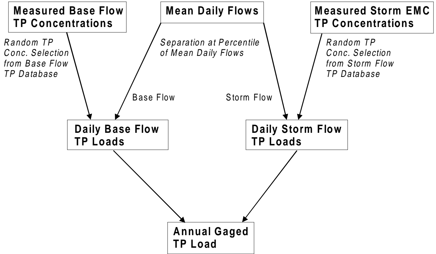
Figure A-1. Schematic of Monte Carlo Method for Gaged TP Load Estimation.
