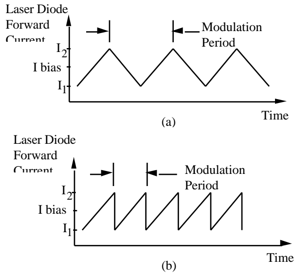
Figure 4.2. Current driver output modulation waveforms, (a) triangular modulation, and (b) sawtooth modulation.
