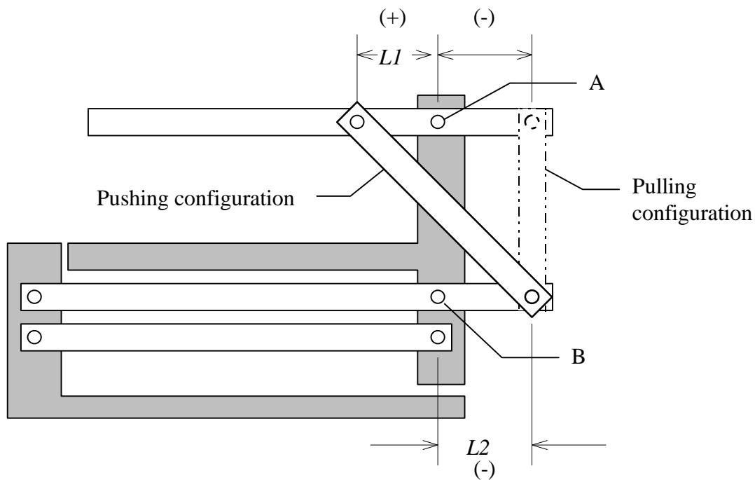
Figure 6-5, Tension Configuration
