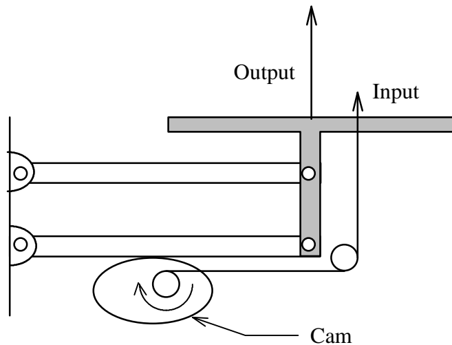
Figure 3-8, Parallel Linkage with a Cam
