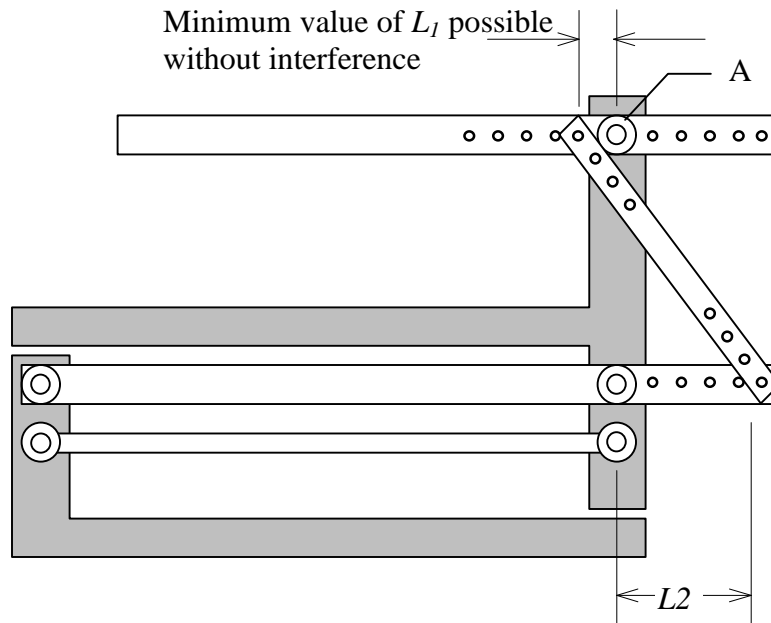
Figure 8-2, Joint Interference
