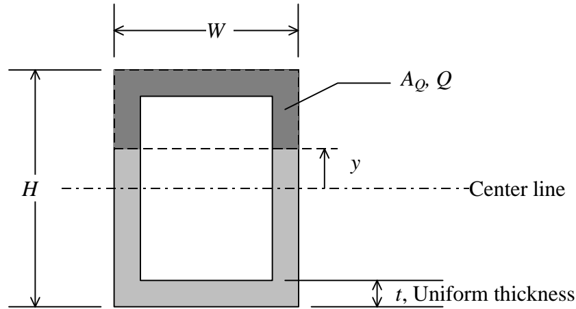
Figure 7-5, Cross Section of Rectangular Tubing
