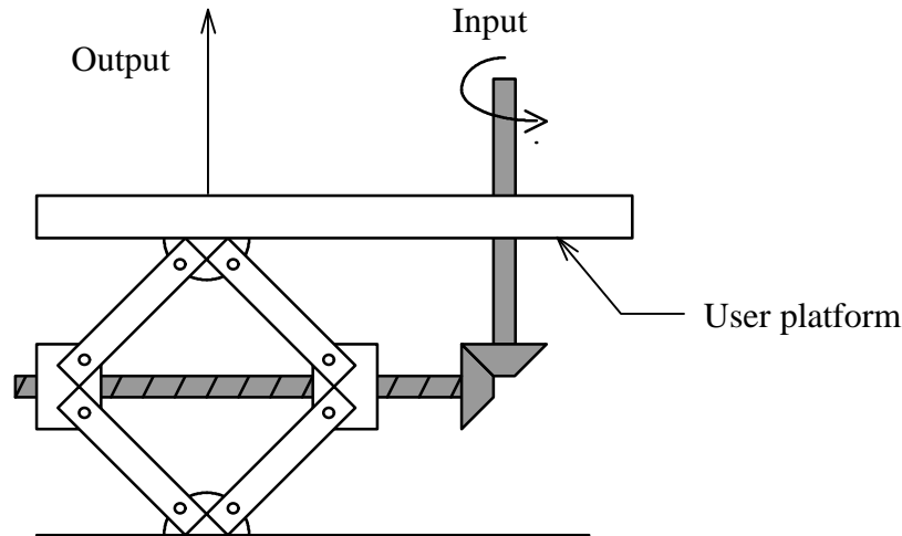
Figure 3-6, Scissors Linkage
