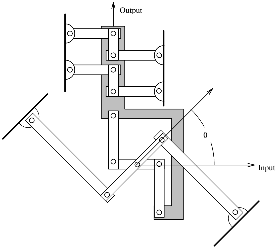
Figure 3-5, Fully Revolute Linkage
