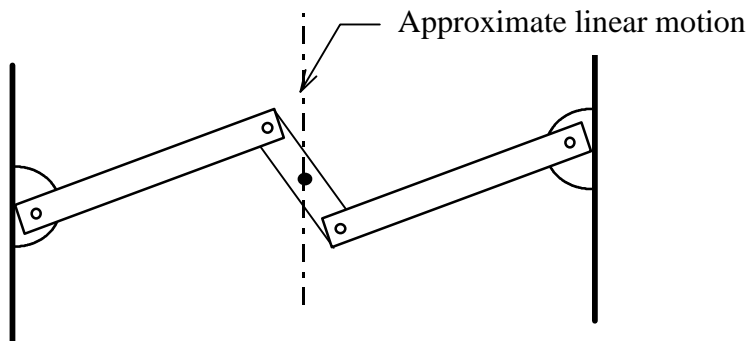
Figure 3-2, Watt's Straight Line Mechanism
