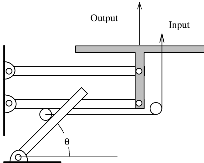
Figure 3-7, Parallel Linkage
