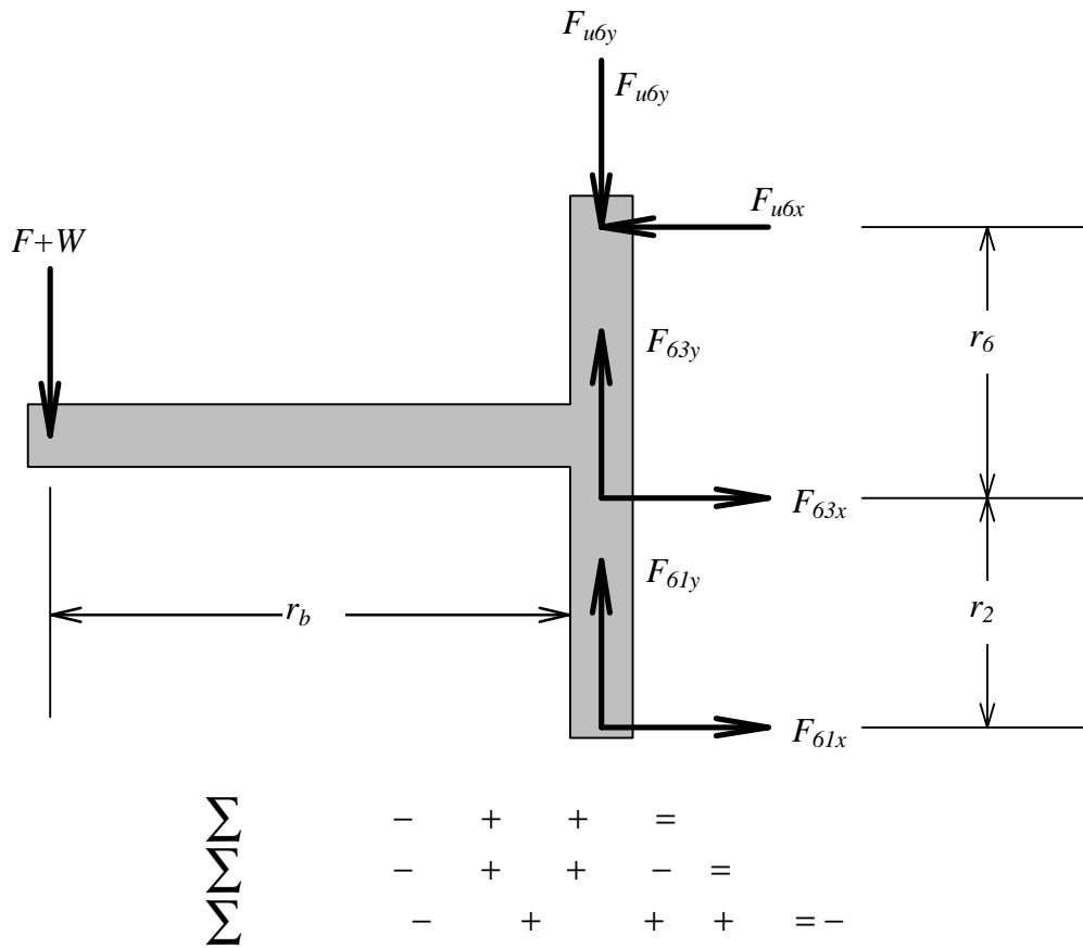
Figure 6-10, Free-Body Diagram of the Platform
