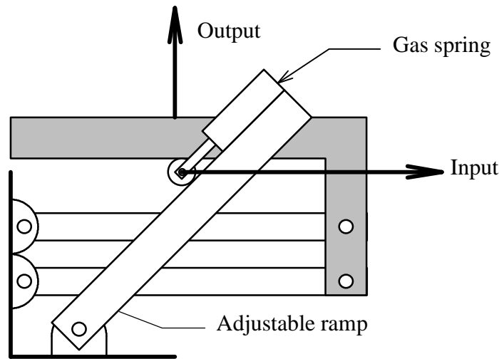
Figure 5-3, Second Roller Schematic
