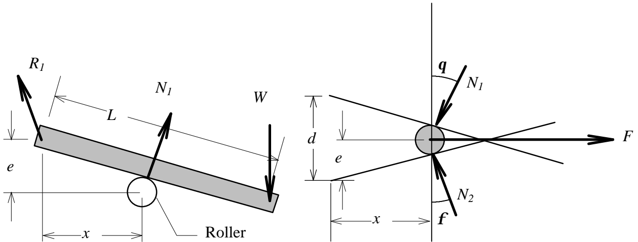
Figure 5-1, Free Body Diagrams of Initial Design
