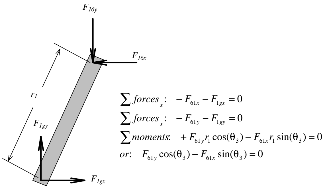
Figure 6-12, Free-Body Diagram of Lower Parallel Link
