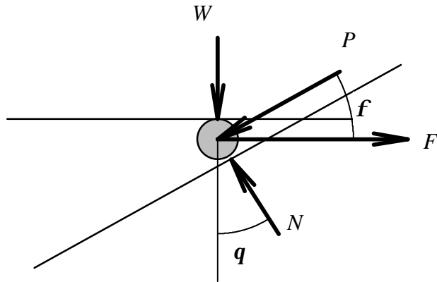
Figure 5-4, Free Body Diagram of Roller Forces
