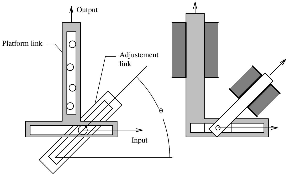
Figure 3-1, Fully Prismatic Linkage
