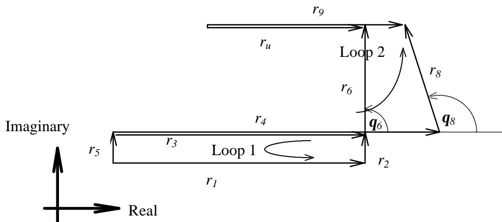
Figure 6-6, Vector Loops For Second Machine
