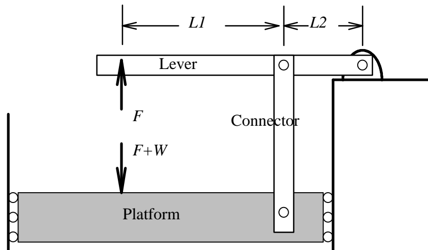
Figure 6-1, Lever Concept
