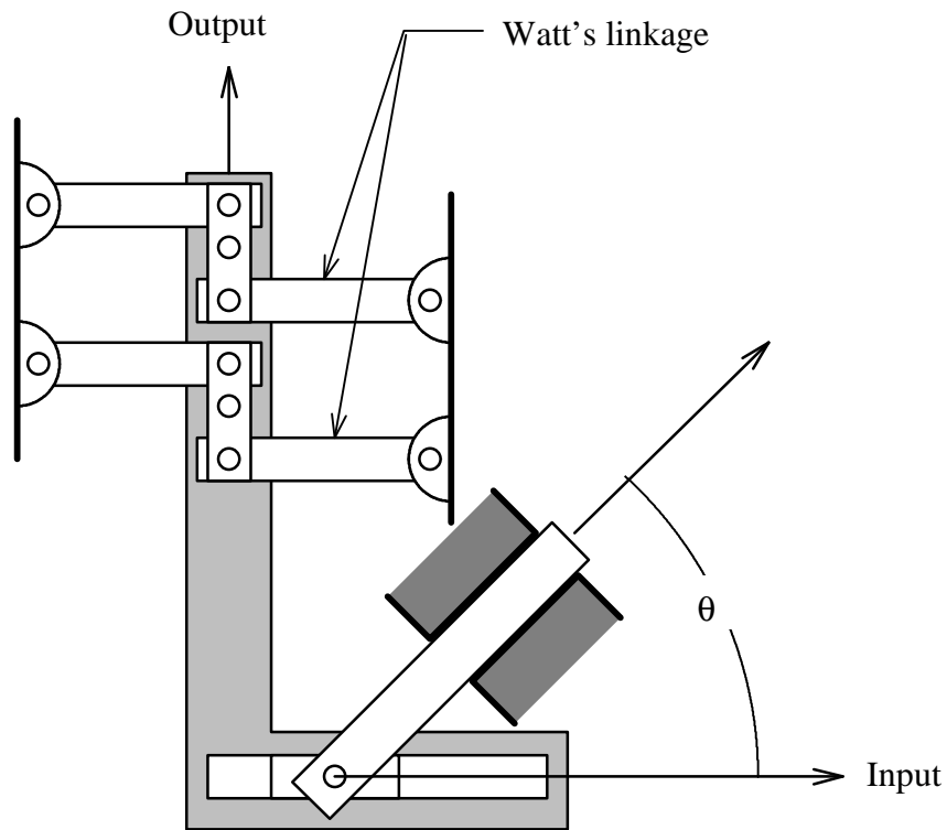
Figure 3-3, One Replace Prismatic
