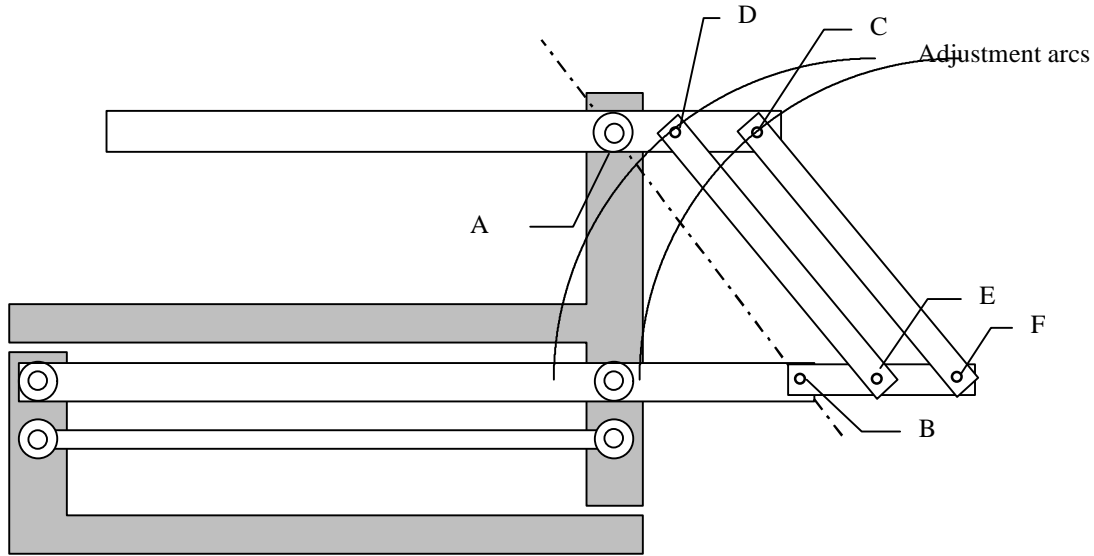
Figure 9-1, Four-Bar Replacement
