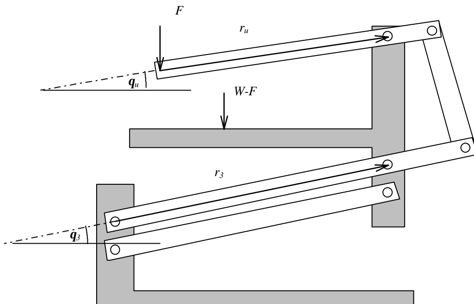
Figure 6-7, Pulling Configuration for Virtual Work
