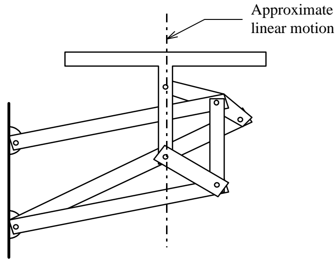
Figure 3-9, Constant orientation linear linkage
