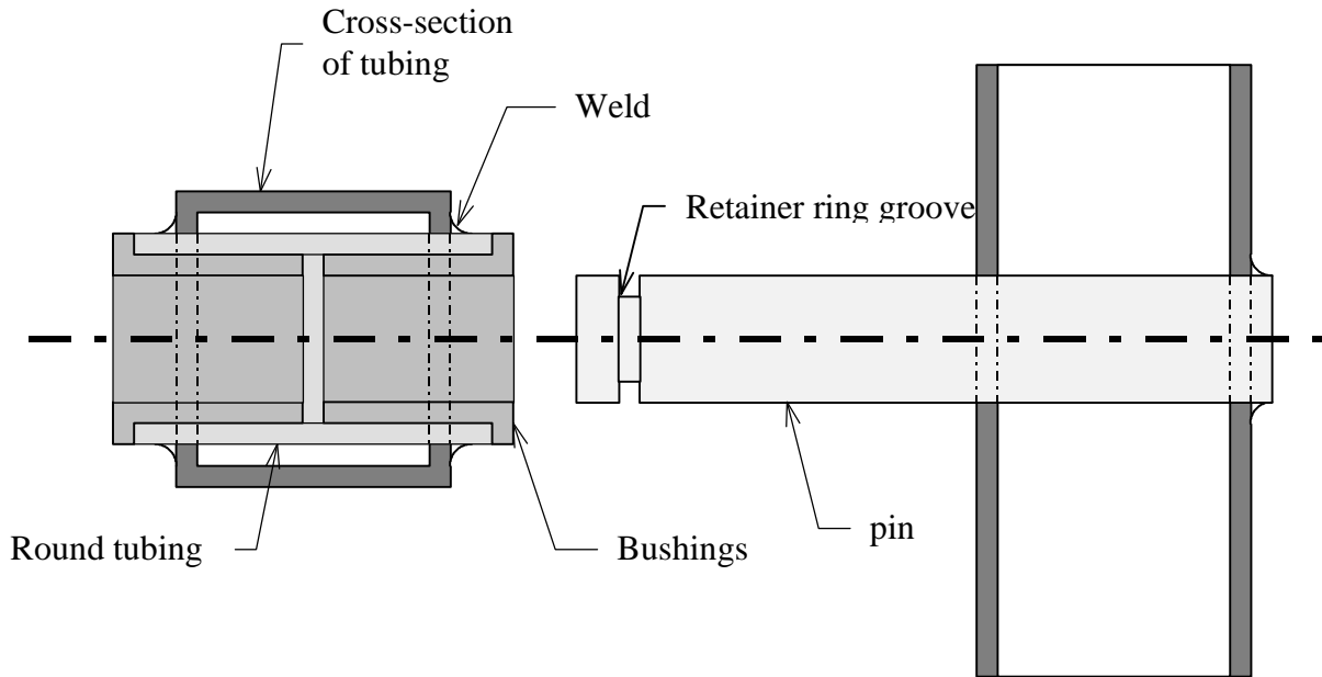
Figure 8-1, Revolute Schematic
