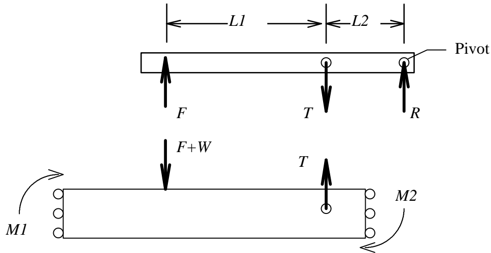
Figure 6-2, Free Body Diagrams of the Lever Concept
