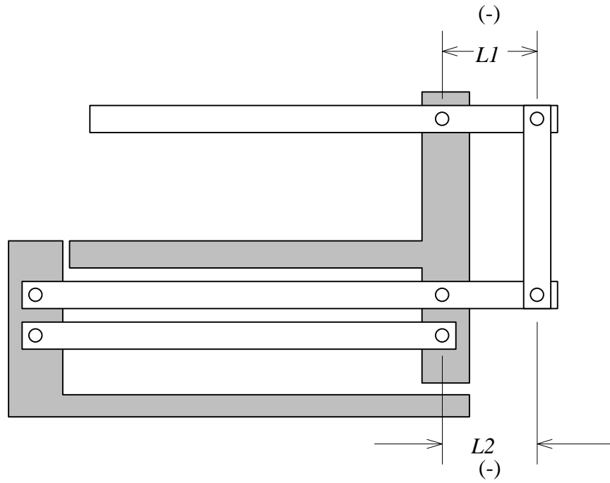
Figure 7-1, Case 1 Pulling Exercise
