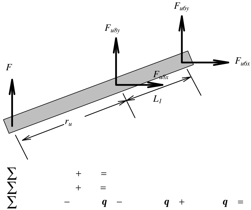
Figure 6-8, Free-Body Diagram of Input Link
