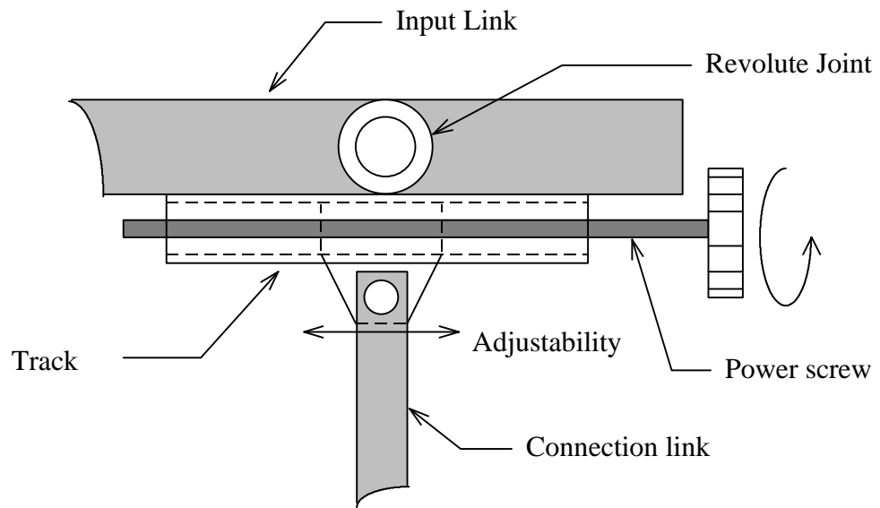
Figure 8-3, New Joint Connection
