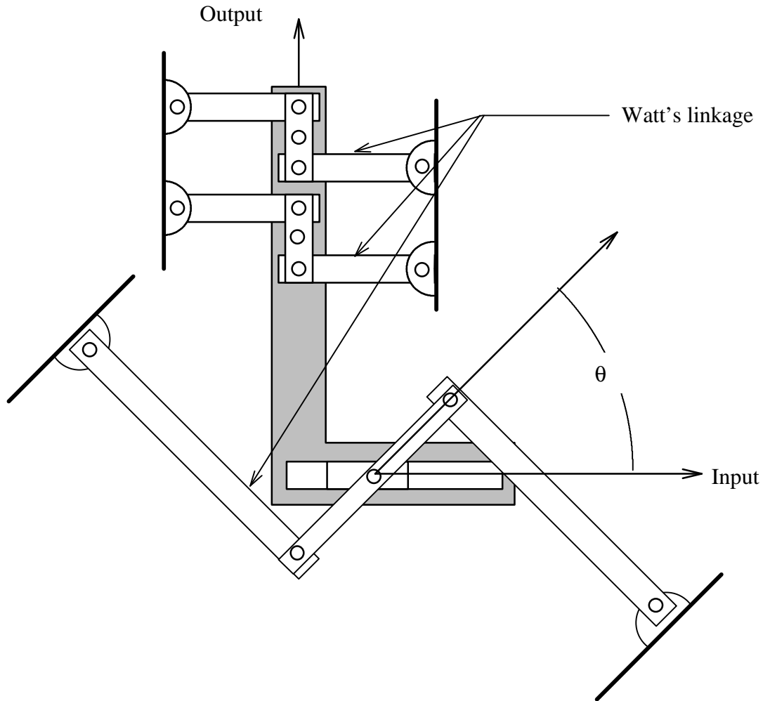
Figure 3-4, Two Replaced Primitives
