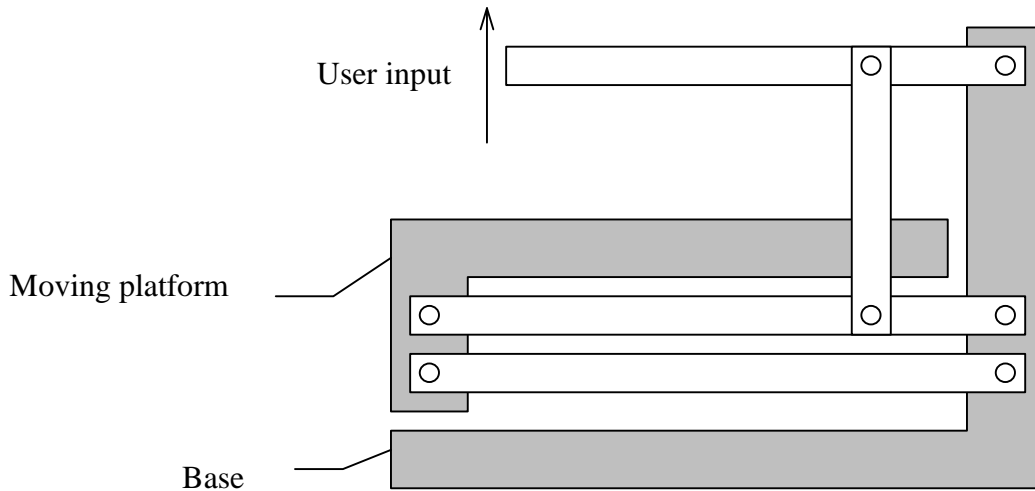
Figure 6-3, Four-Bar Lever Concept
