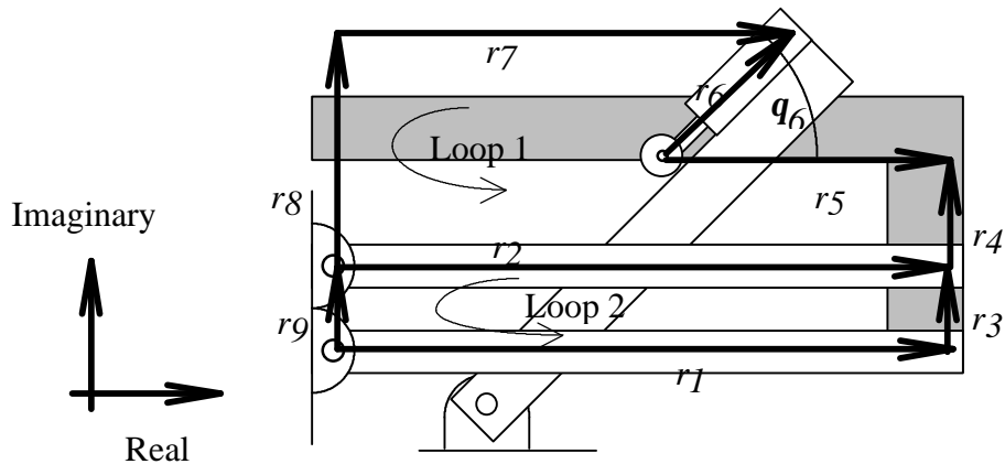
Figure 5-6, Loop Vectors
