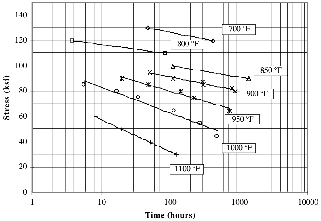
Figure 4.39 Time Required for a HA50HS Specimen to Fracture as a Function of Applied Stress and Temperature.
