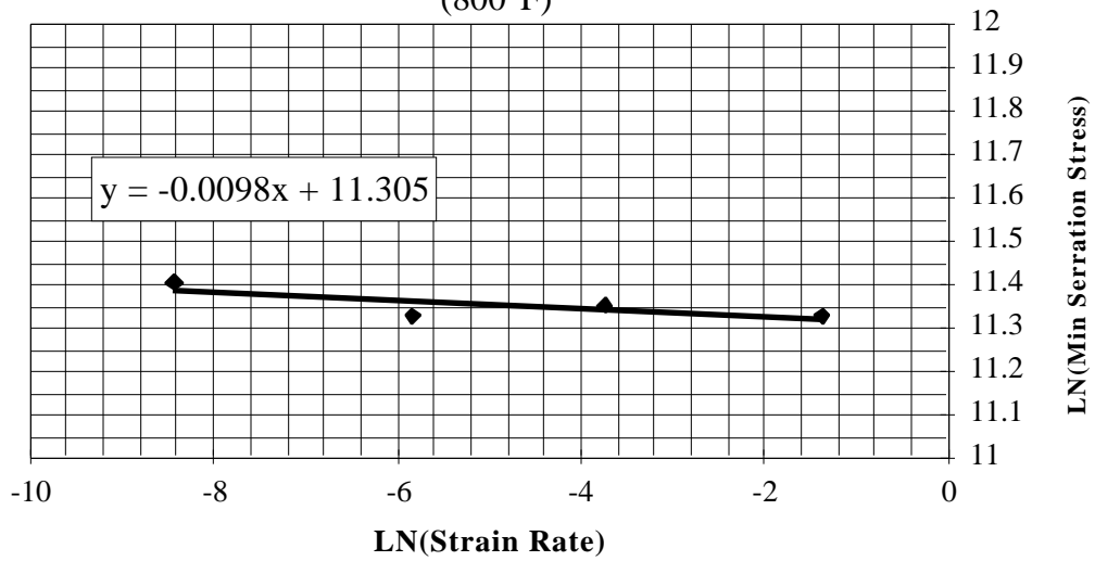
Figure 4.13 Strain Rate Sensitivity Curves at 800°F Corresponding to the Maximum and Minimum Serration Stress Levels.
