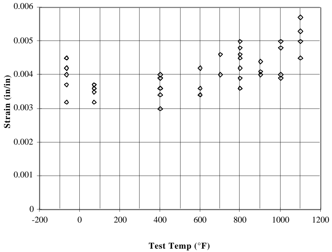
Figure 4.6 Elastic Strain Versus Test Temperature of HA50HS Specimens Tested in the 45 Degree Orientation.
