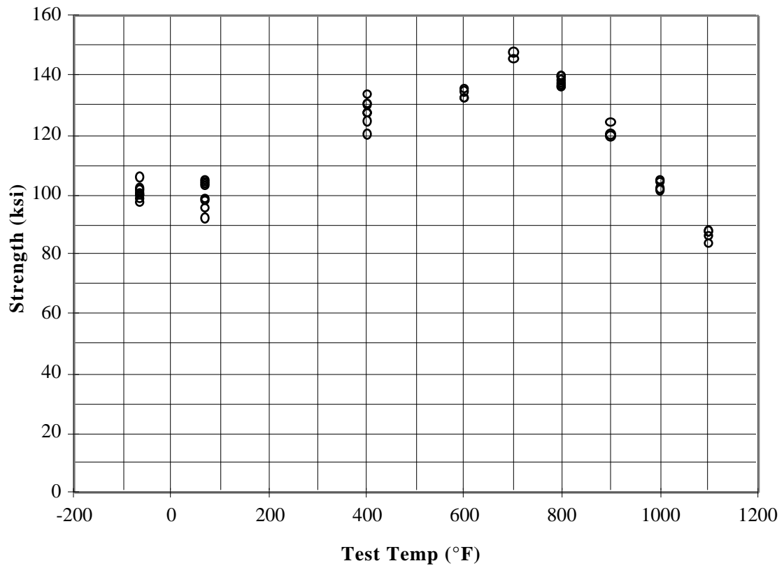
Figure 4.10 Ultimate Tensile Strength Versus Test Temperature of HA50HS Specimens Tested in the 45 Degree Orientation.
