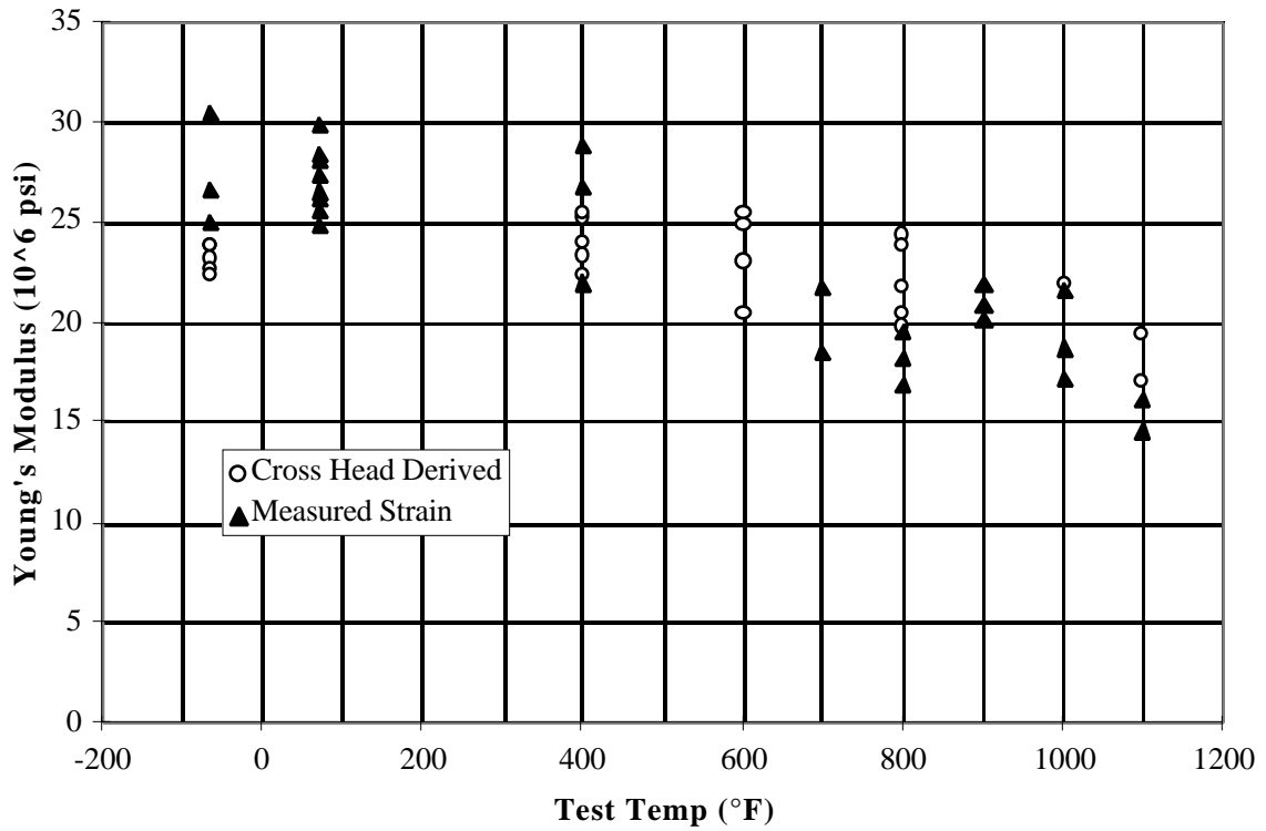
Figure 4.5 Elastic Modulus Versus Temperature for Hiperco® Alloy 50HS as Determined for the 45 Degree Orientation to Rolling Direction.
