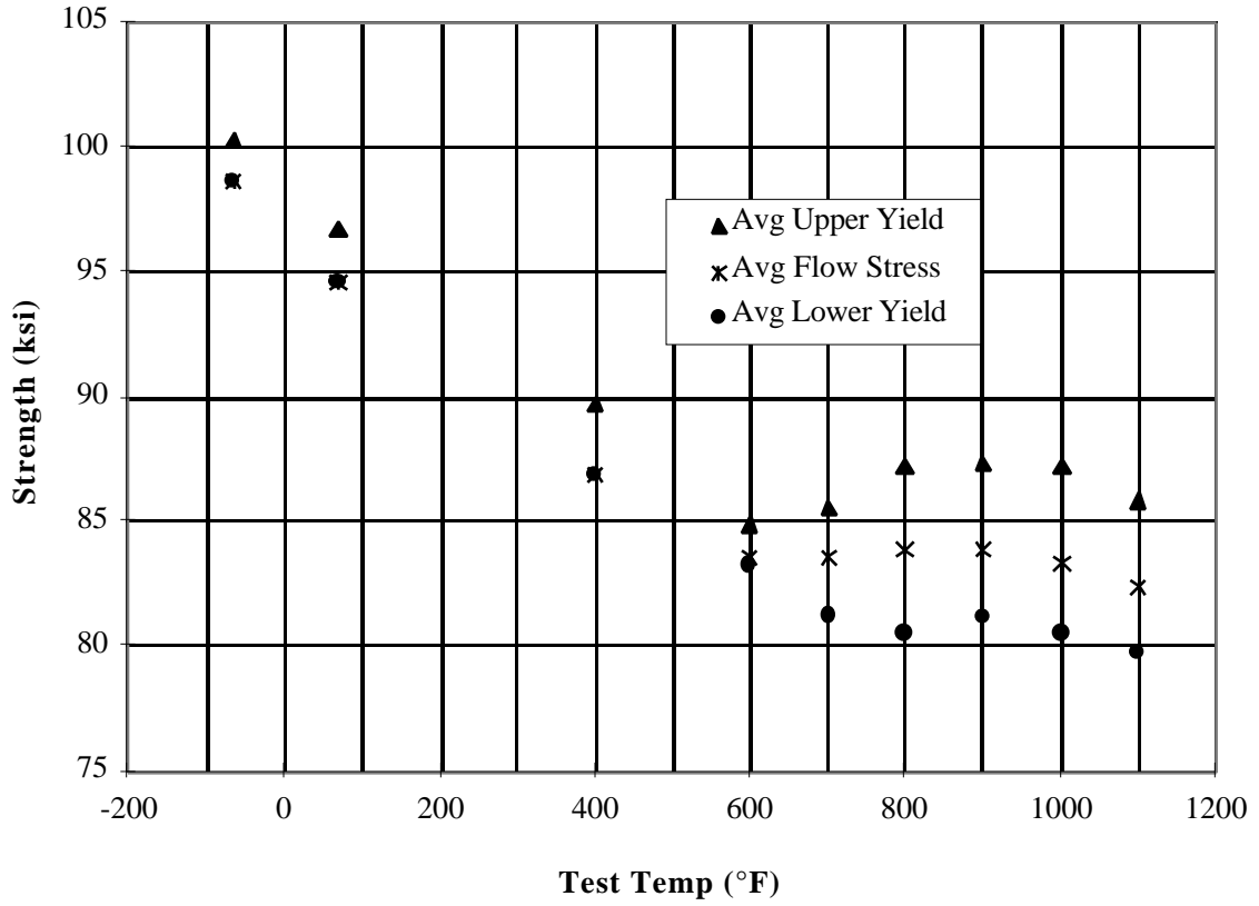
Figure 4.8 Average Yield Strengths of HA50HS Specimens Tested in the 45 Degree Orientation.
