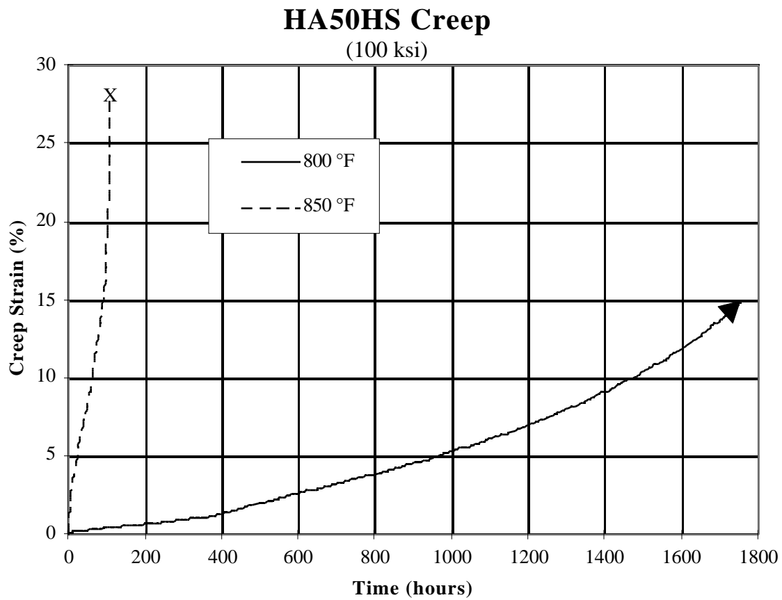
Figure 4.27 Creep Strain Versus Time Response of HA50HS Specimens Tested at 100 ksi.
