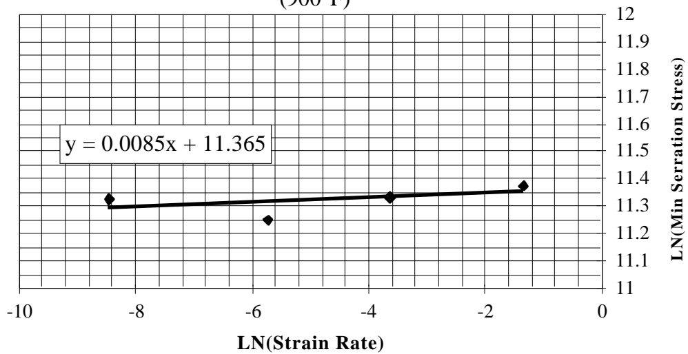
Figure 4.14 Strain Rate Sensitivity Curves at 900°F Corresponding to the Maximum and Minimum Serration Stress Levels.
