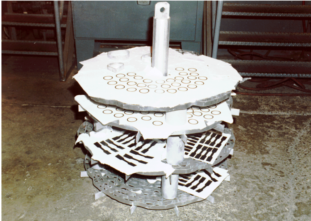
Figure 3.1 Furnace Rack Used by Wall Colmonoy to Heat Treat Various Iron-Cobalt Test Specimens.
