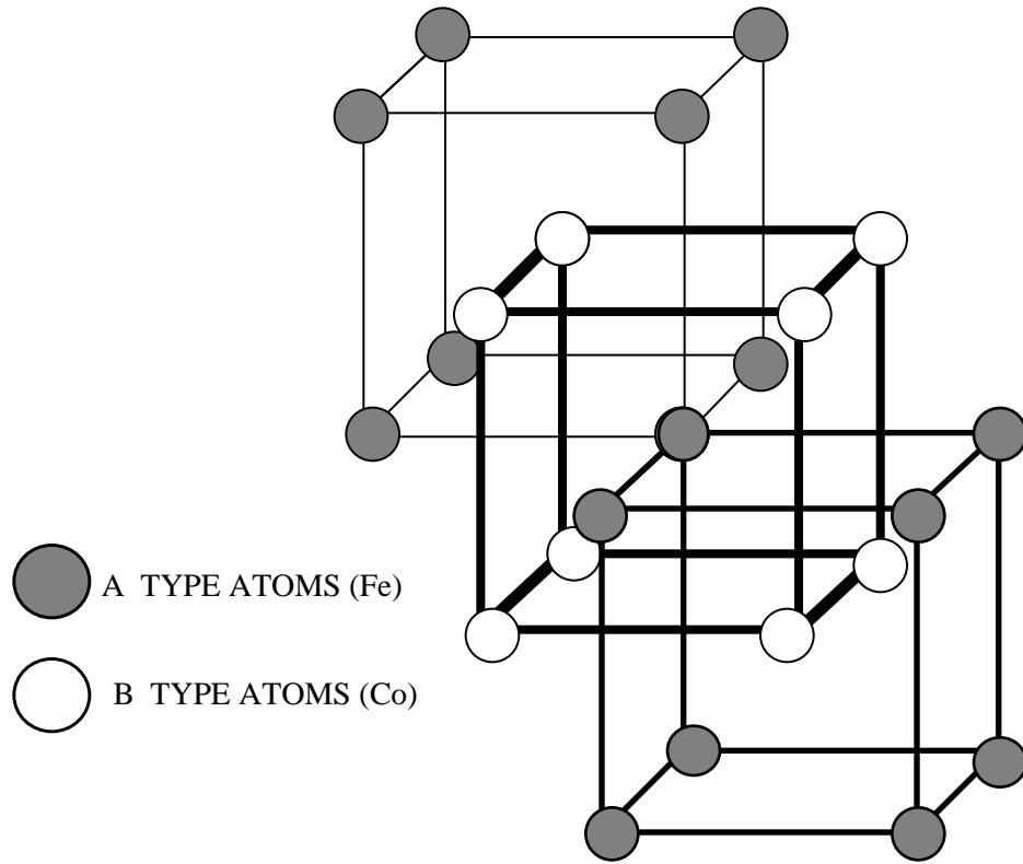
Figure 2.1 B2 Ordered Microstructure.
