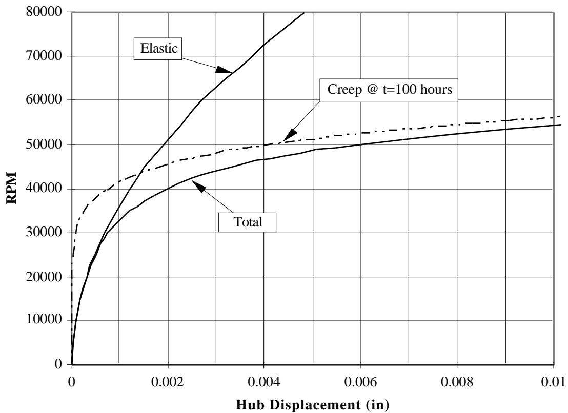
Figure 5.15 Calculated Elastic and Creep Deformations and Estimated Total Displacement of the Hub Radius of Rotor Configuration #3, Tested at 1000°F, as a Function of the Rotor Speed.
