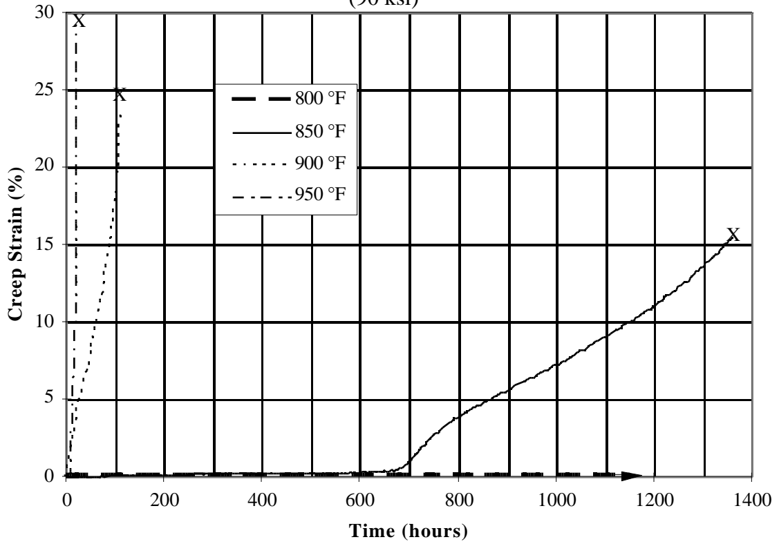
Figure 4.26 Creep Strain Versus Time Response of HA50HS Specimens Tested at 90 ksi.
