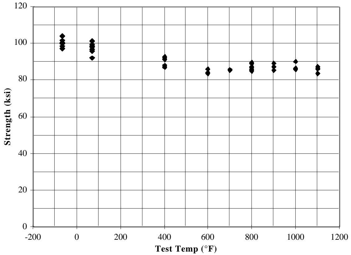
Figure 4.7 Upper Yield Strength Versus Test Temperature of HA50HS Specimens Tested in the 45 Degree Orientation.
