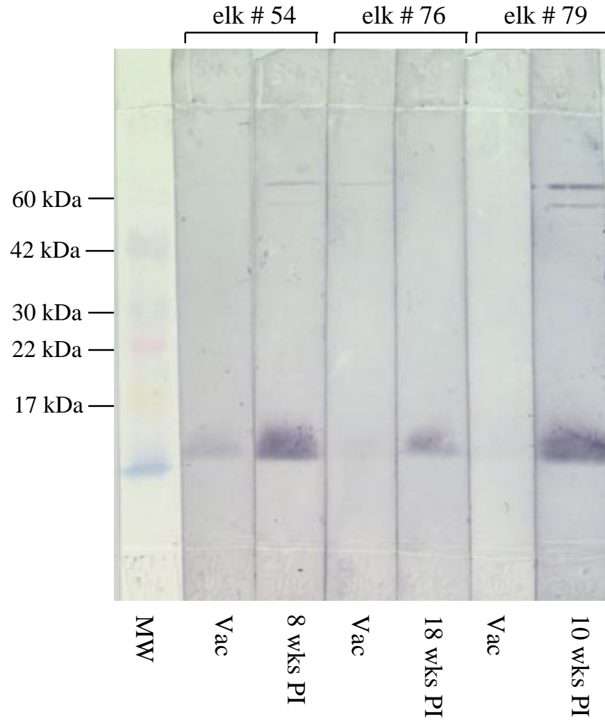
Figure 2.20. Western blot of biobullet elk #54, 76, and 79 against whole cell RB51 antigen developed with polyclonal anti-bovine IgG (Cappel - West Chester, PA).
